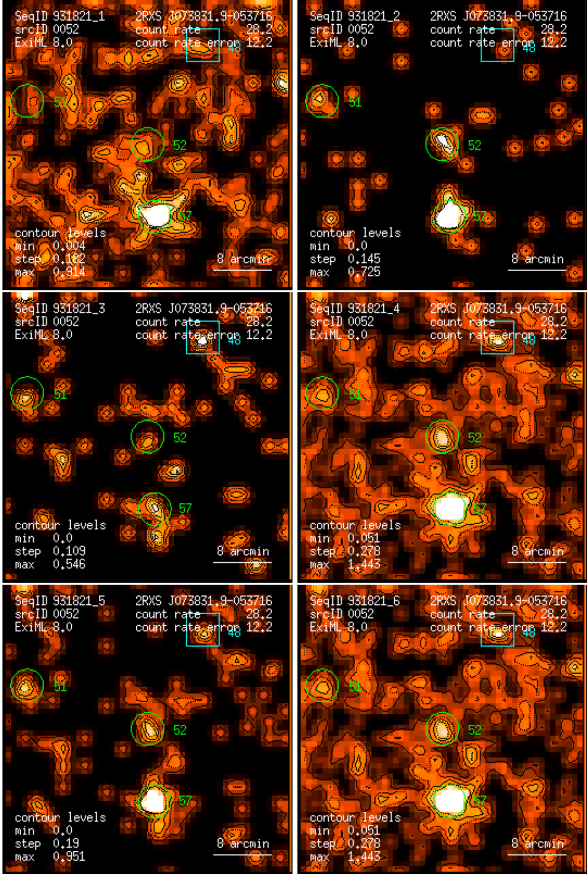
Figure 52: RASS 931821: detection 0052: band rate images, Gaussian filter: (1) PSPC channels 11 – 41, (2) 52 – 90, (3) 91 – 201, (4) 11 – 235, (5) 52 – 201, (6) 11 – 201. Broad band rates in counts/ks. Band rate contour levels in counts/ks/arcmin 2 .
