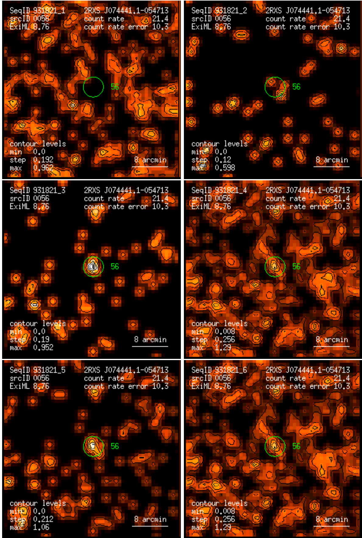
Figure 56: RASS 931821: detection 0056: band rate images, Gaussian filter: (1) PSPC channels 11 – 41, (2) 52 – 90, (3) 91 – 201, (4) 11 – 235, (5) 52 – 201, (6) 11 – 201. Broad band rates in counts/ks. Band rate contour levels in counts/ks/arcmin 2 .
