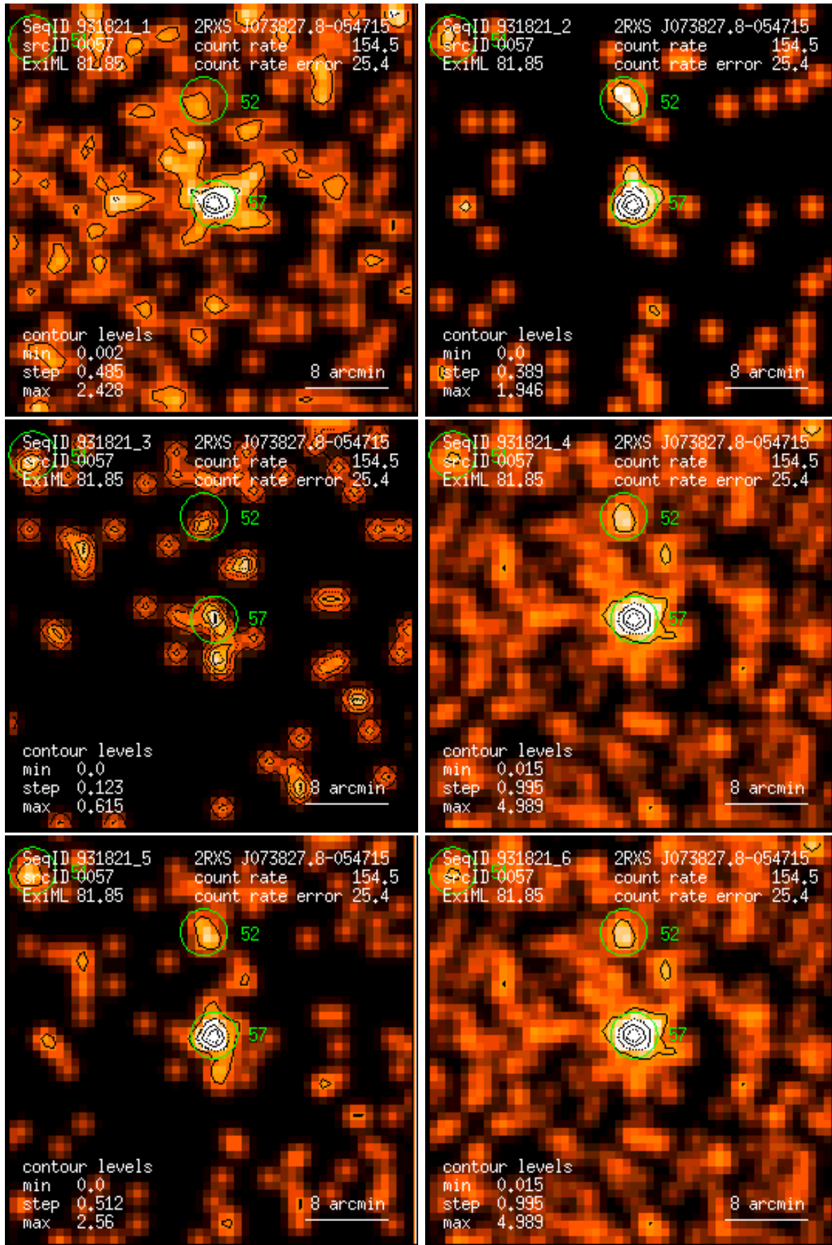
Figure 57: RASS 931821: detection 0057: band rate images, Gaussian filter: (1) PSPC channels 11 – 41, (2) 52 – 90, (3) 91 – 201, (4) 11 – 235, (5) 52 – 201, (6) 11 – 201. Broad band rates in counts/ks. Band rate contour levels in counts/ks/arcmin 2 .
