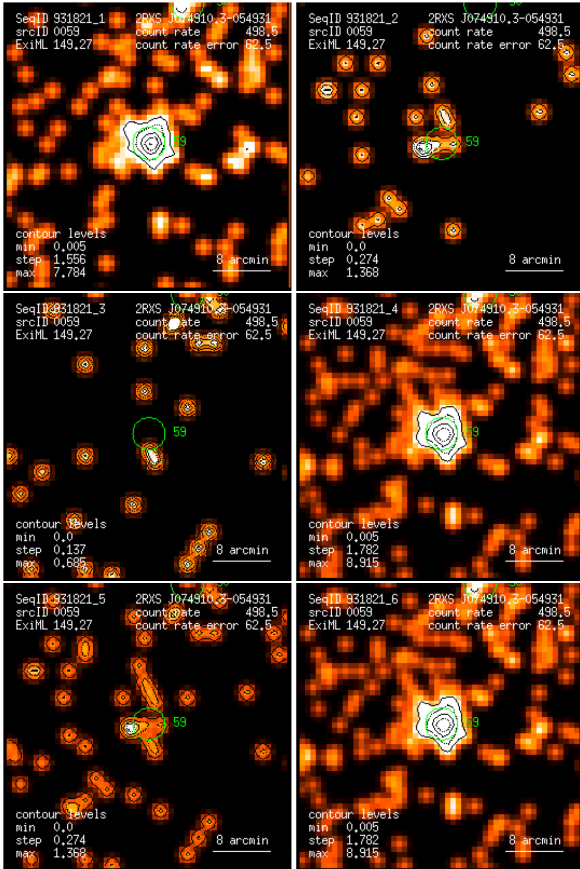
Figure 59: RASS 931821: detection 0059: band rate images, Gaussian filter: (1) PSPC channels 11 – 41, (2) 52 – 90, (3) 91 – 201, (4) 11 – 235, (5) 52 – 201, (6) 11 – 201. Broad band rates in counts/ks. Band rate contour levels in counts/ks/arcmin 2 .
