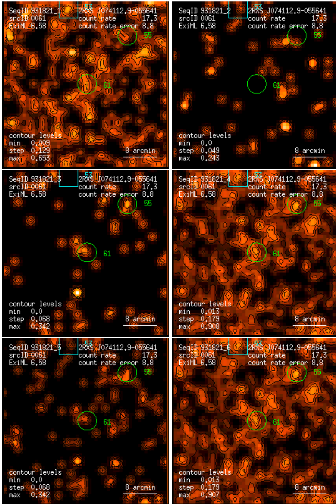
Figure 61: RASS 931821: detection 0061: band rate images, Gaussian filter: (1) PSPC channels 11 – 41, (2) 52 – 90, (3) 91 – 201, (4) 11 – 235, (5) 52 – 201, (6) 11 – 201. Broad band rates in counts/ks. Band rate contour levels in counts/ks/arcmin 2 .
