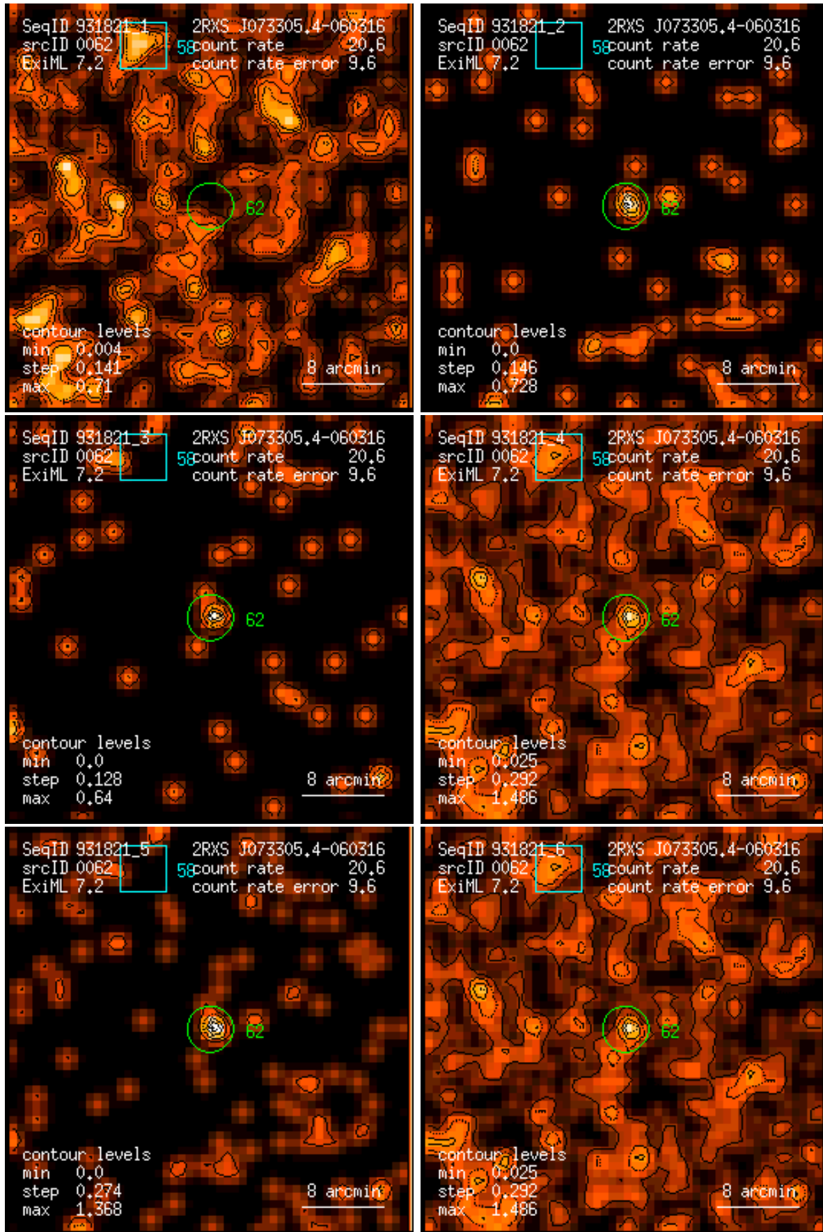
Figure 62: RASS 931821: detection 0062: band rate images, Gaussian filter: (1) PSPC channels 11 – 41, (2) 52 – 90, (3) 91 – 201, (4) 11 – 235, (5) 52 – 201, (6) 11 – 201. Broad band rates in counts/ks. Band rate contour levels in counts/ks/arcmin 2 .
