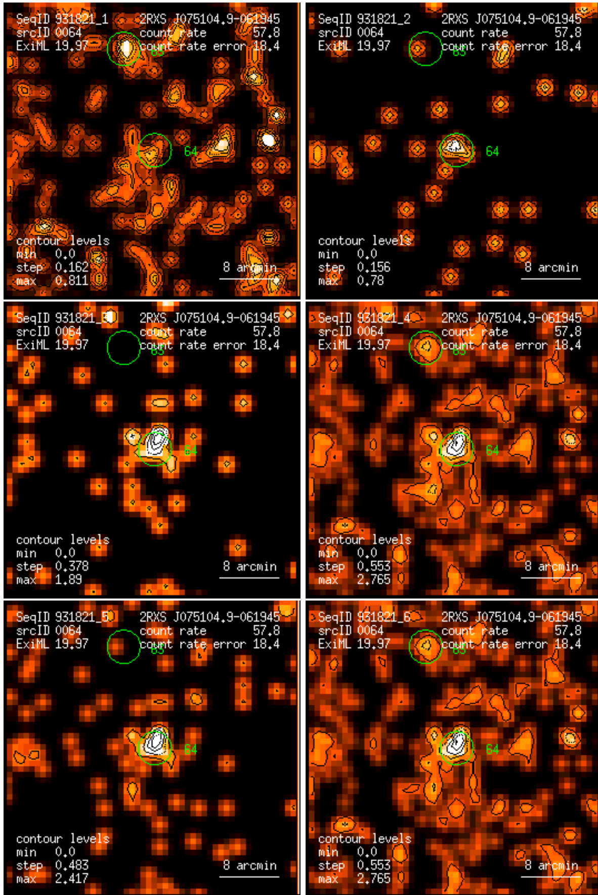
Figure 64: RASS 931821: detection 0064: band rate images, Gaussian filter: (1) PSPC channels 11 – 41, (2) 52 – 90, (3) 91 – 201, (4) 11 – 235, (5) 52 – 201, (6) 11 – 201. Broad band rates in counts/ks. Band rate contour levels in counts/ks/arcmin 2 .
