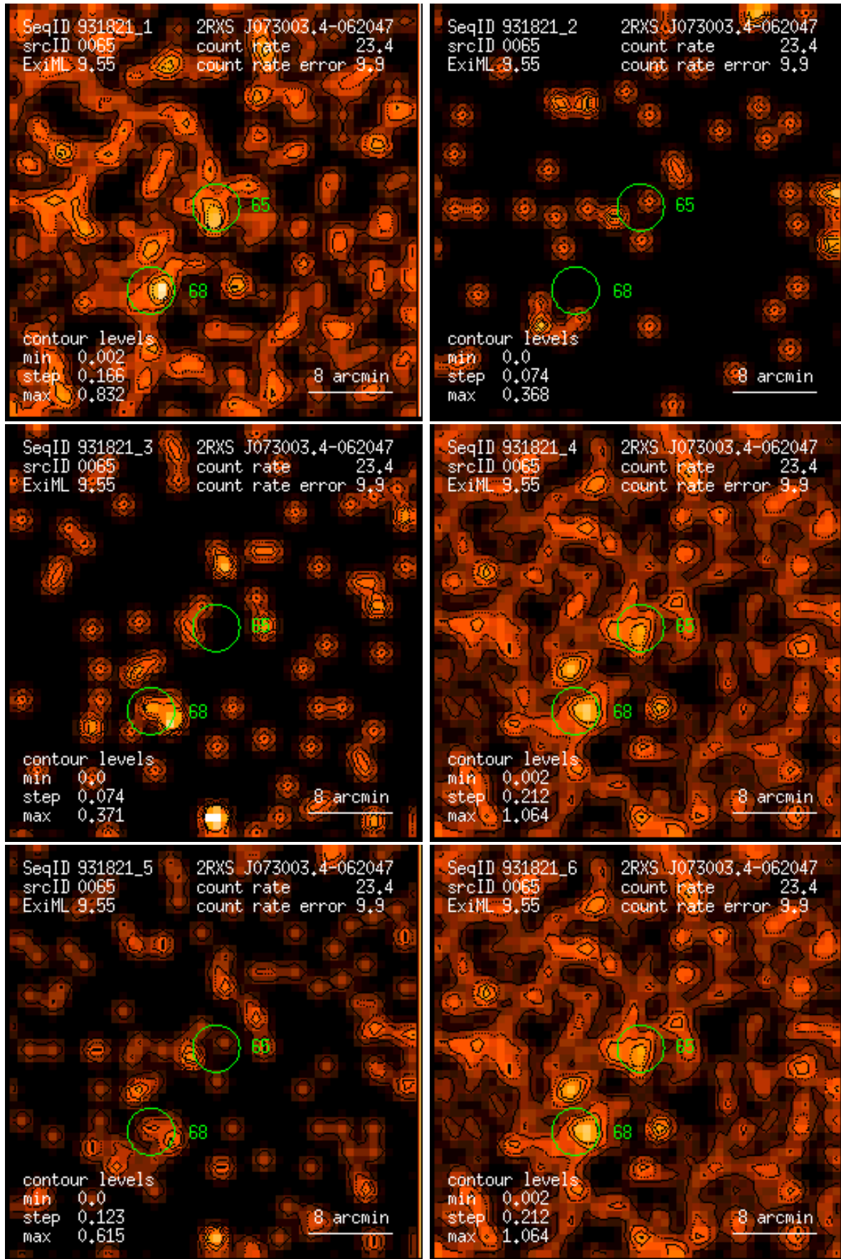
Figure 65: RASS 931821: detection 0065: band rate images, Gaussian filter: (1) PSPC channels 11 – 41, (2) 52 – 90, (3) 91 – 201, (4) 11 – 235, (5) 52 – 201, (6) 11 – 201. Broad band rates in counts/ks. Band rate contour levels in counts/ks/arcmin 2 .
