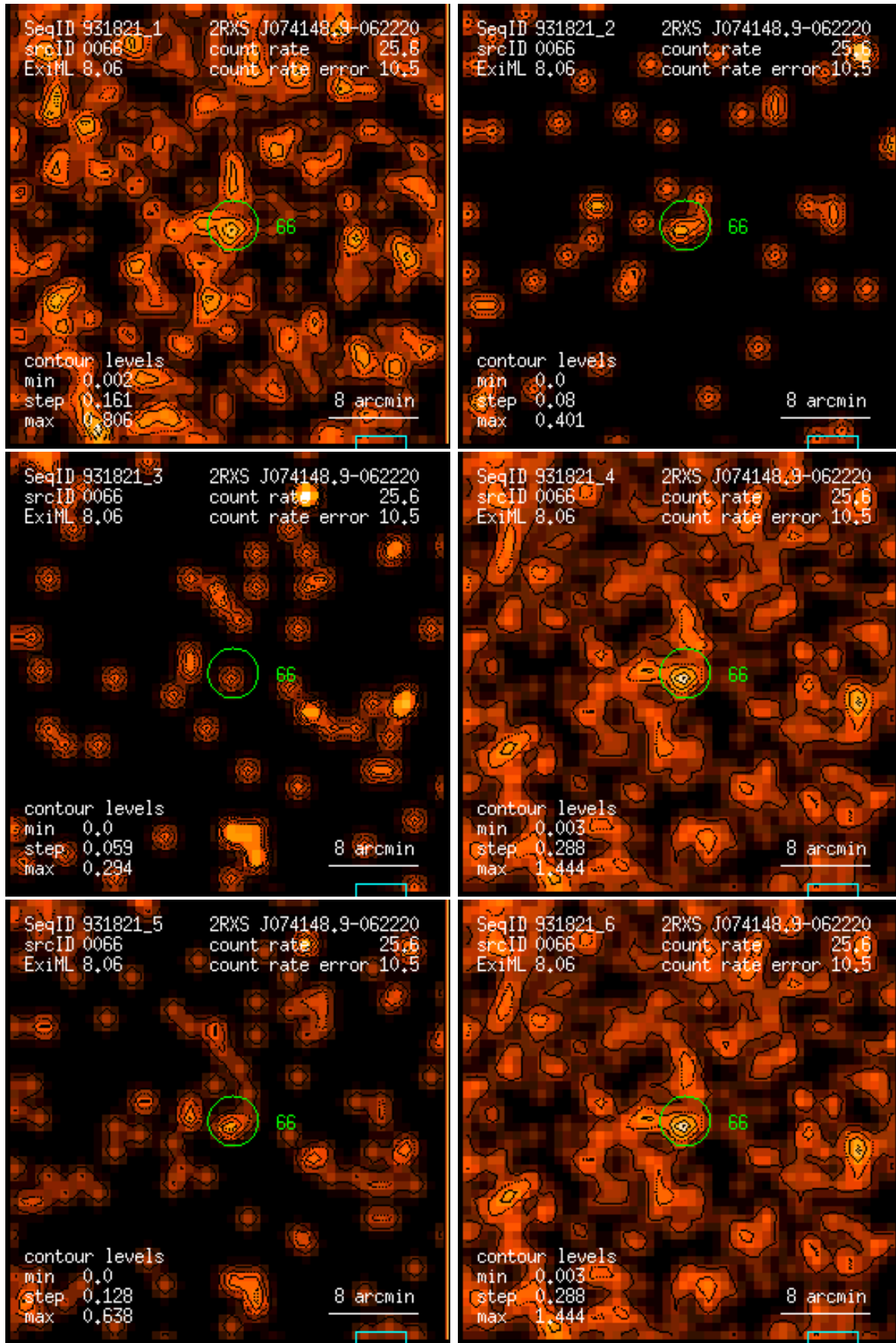
Figure 66: RASS 931821: detection 0066: band rate images, Gaussian filter: (1) PSPC channels 11 – 41, (2) 52 – 90, (3) 91 – 201, (4) 11 – 235, (5) 52 – 201, (6) 11 – 201. Broad band rates in counts/ks. Band rate contour levels in counts/ks/arcmin 2 .
