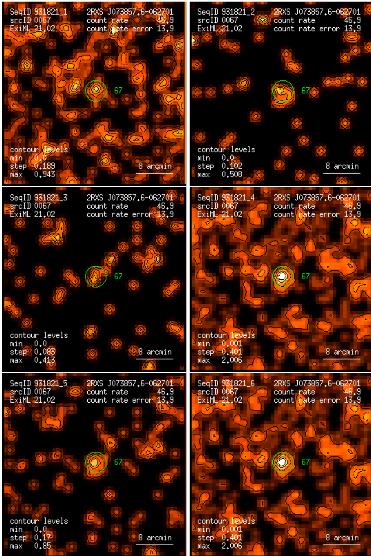
Figure 67: RASS 931821: detection 0067: band rate images, Gaussian filter: (1) PSPC channels 11 – 41, (2) 52 – 90, (3) 91 – 201, (4) 11 – 235, (5) 52 – 201, (6) 11 – 201. Broad band rates in counts/ks. Band rate contour levels in counts/ks/arcmin 2 .
