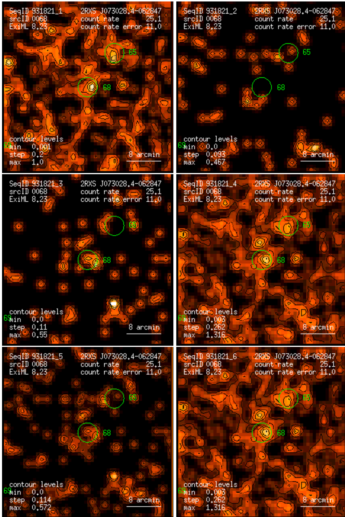
Figure 68: RASS 931821: detection 0068: band rate images, Gaussian filter: (1) PSPC channels 11 – 41, (2) 52 – 90, (3) 91 – 201, (4) 11 – 235, (5) 52 – 201, (6) 11 – 201. Broad band rates in counts/ks. Band rate contour levels in counts/ks/arcmin 2 .
