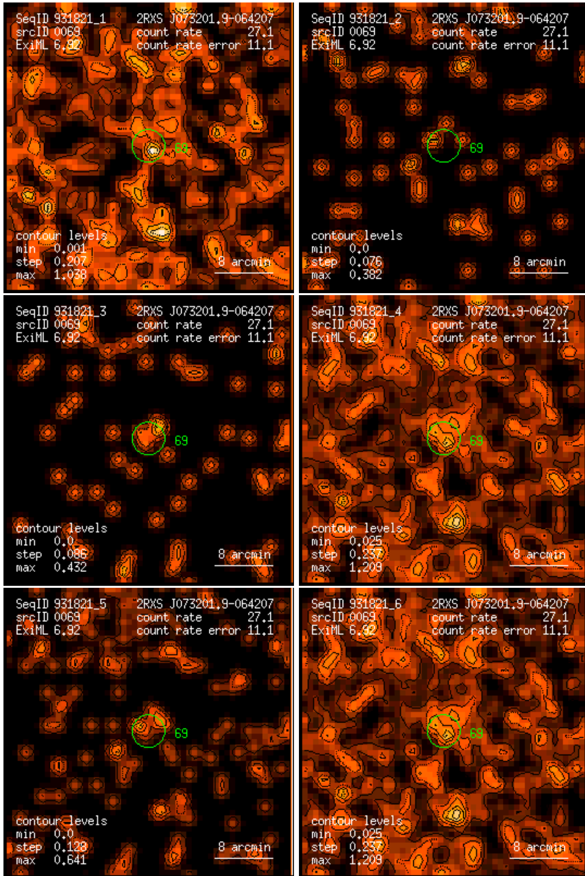
Figure 69: RASS 931821: detection 0069: band rate images, Gaussian filter: (1) PSPC channels 11 – 41, (2) 52 – 90, (3) 91 – 201, (4) 11 – 235, (5) 52 – 201, (6) 11 – 201. Broad band rates in counts/ks. Band rate contour levels in counts/ks/arcmin 2 .
