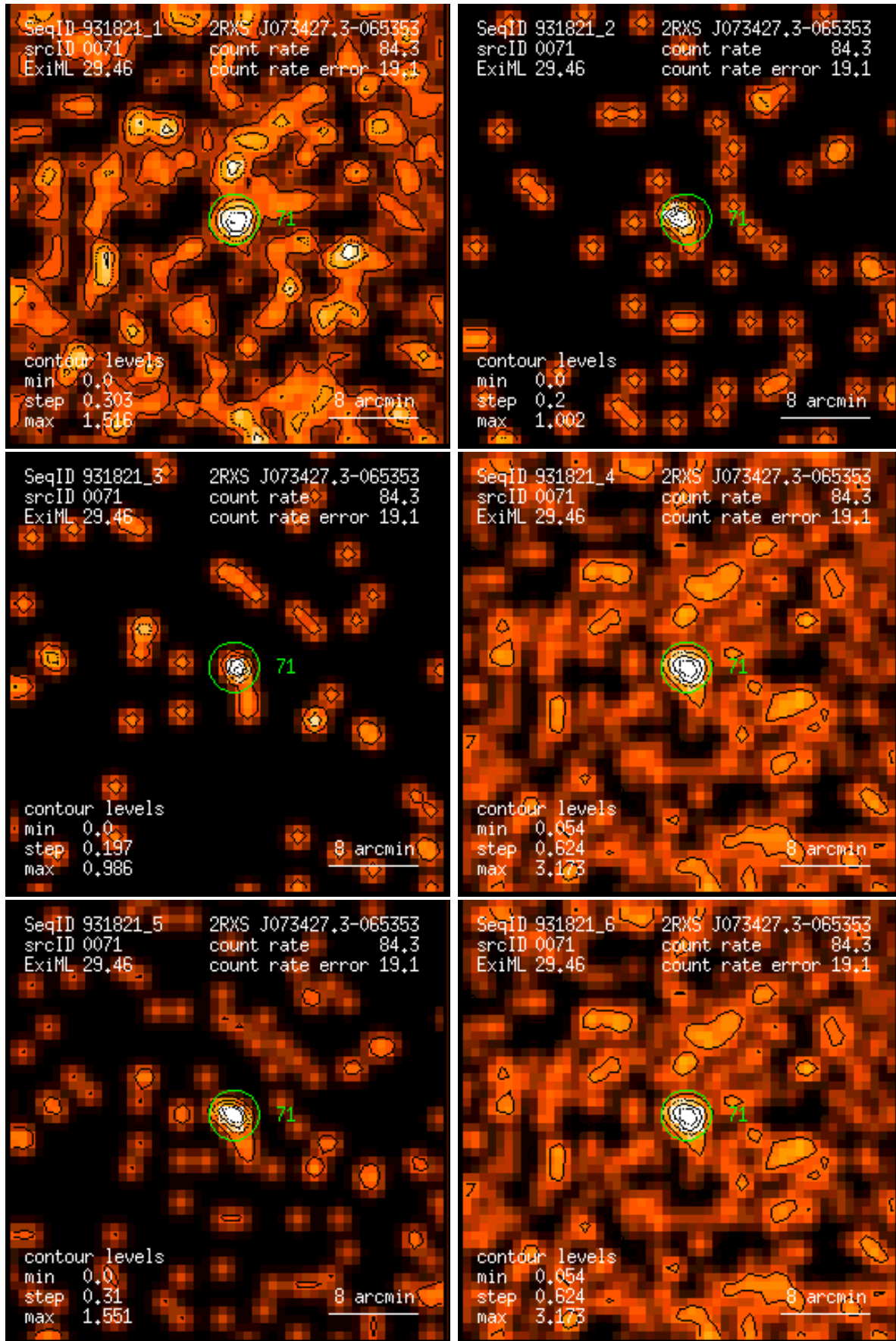
Figure 71: RASS 931821: detection 0071: band rate images, Gaussian filter: (1) PSPC channels 11 – 41, (2) 52 – 90, (3) 91 – 201, (4) 11 – 235, (5) 52 – 201, (6) 11 – 201. Broad band rates in counts/ks. Band rate contour levels in counts/ks/arcmin 2 .
