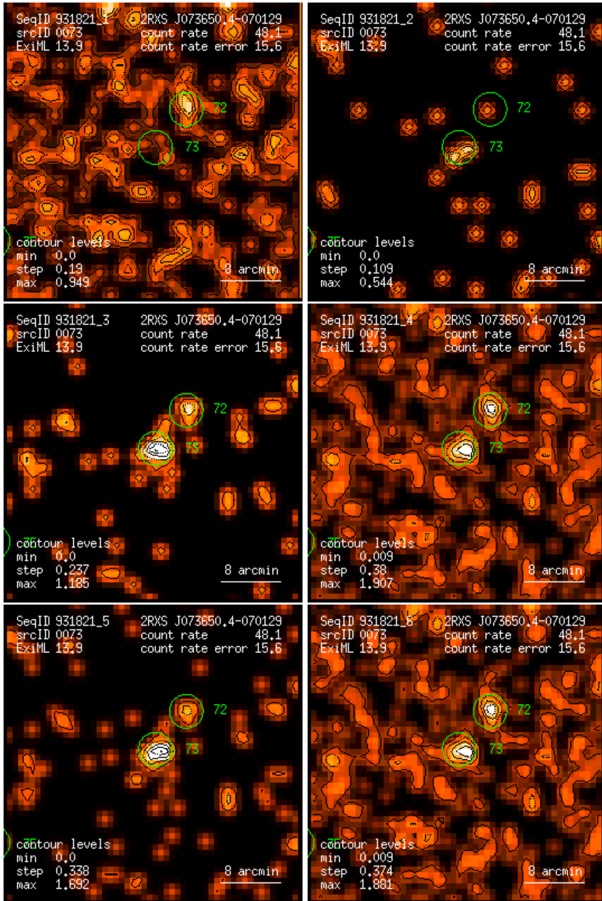
Figure 73: RASS 931821: detection 0073: band rate images, Gaussian filter: (1) PSPP channels 11 – 41, (2) 52 – 90, (3) 91 – 201, (4) 11 – 235, (5) 52 – 201, (6) 11 – 201. Broad band rates in counts/ks. Band rate contour levels in counts/ks/arcmin 2 .
