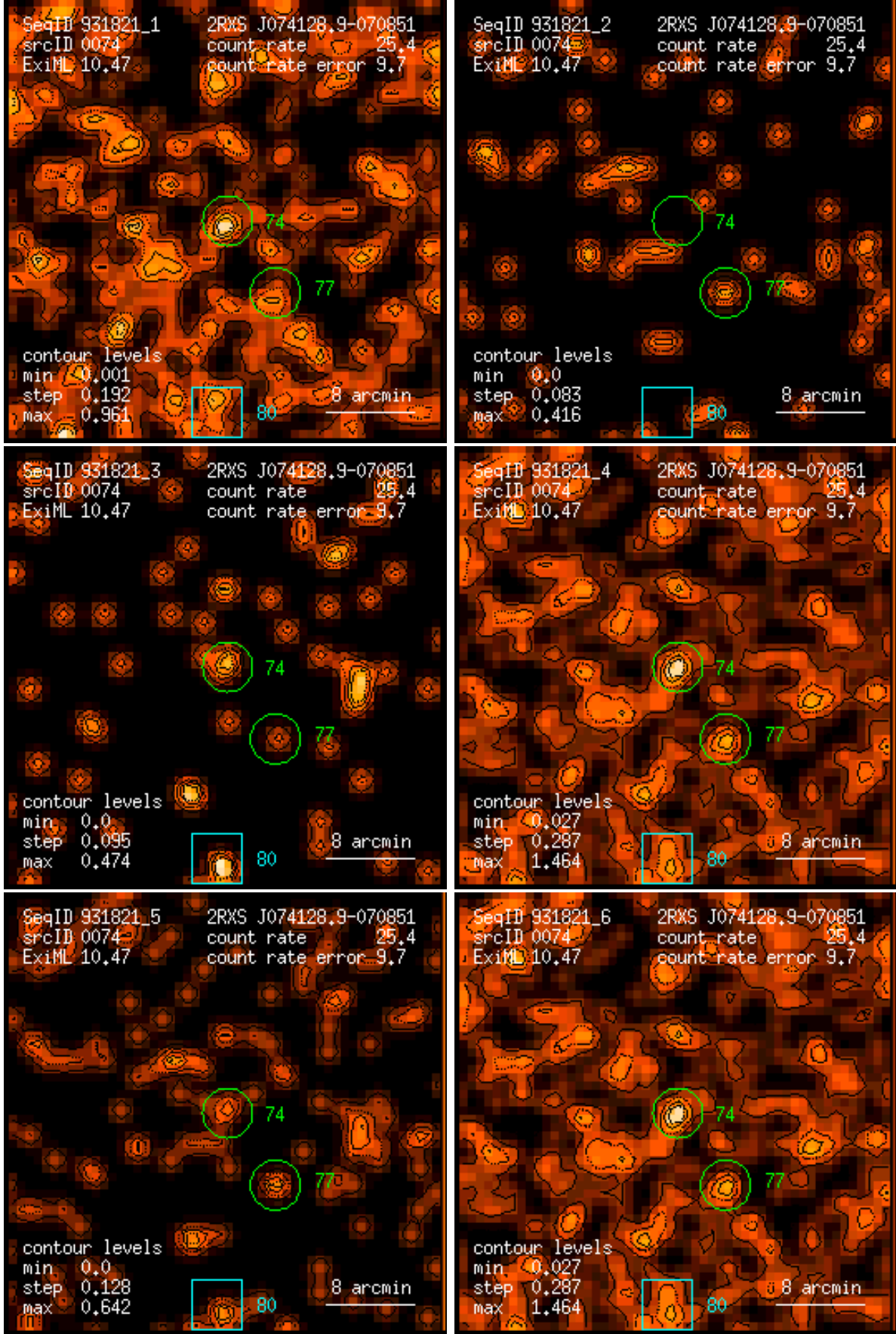
Figure 74: RASS 931821: detection 0074: band rate images, Gaussian filter: (1) PSPC channels 11 – 41, (2) 52 – 90, (3) 91 – 201, (4) 11 – 235, (5) 52 – 201, (6) 11 – 201. Broad band rates in counts/ks. Band rate contour levels in counts/ks/arcmin 2 .
