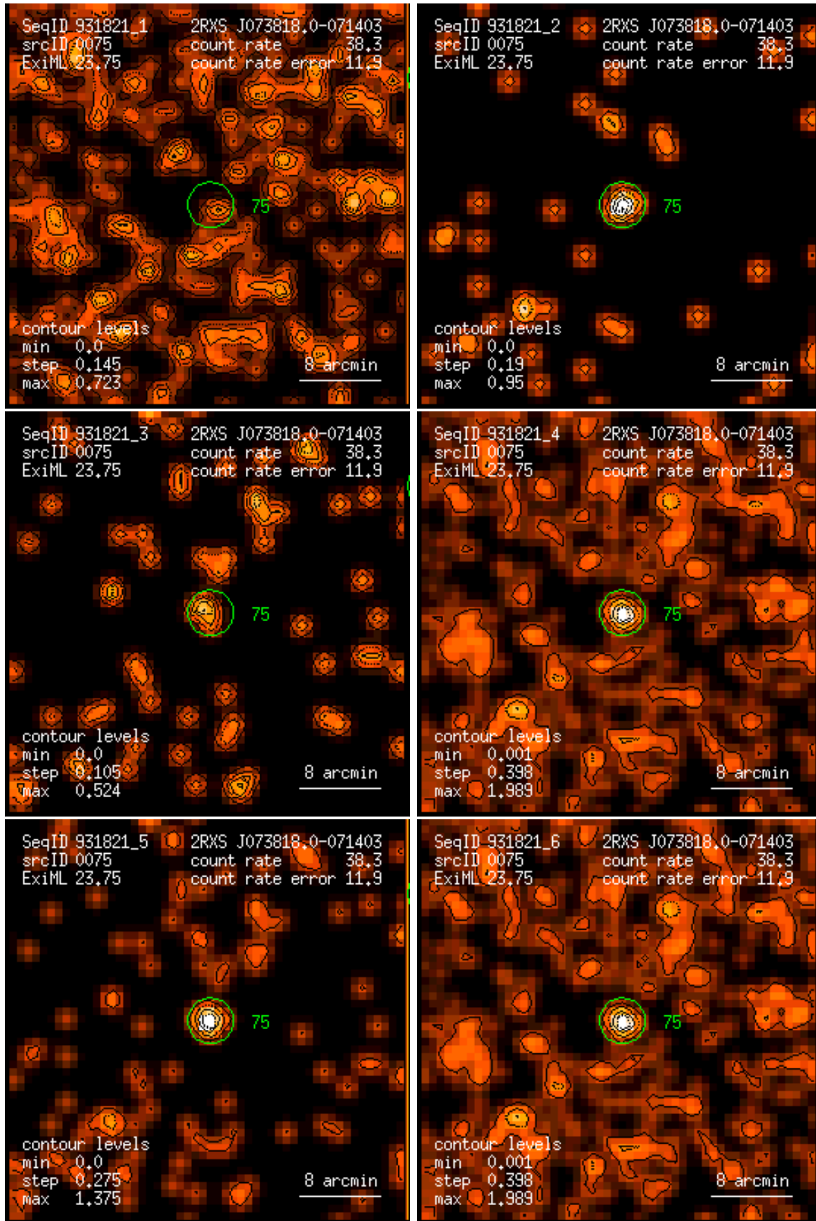
Figure 75: RASS 931821: detection 0075: band rate images, Gaussian filter: (1) PSPC channels 11 – 41, (2) 52 – 90, (3) 91 – 201, (4) 11 – 235, (5) 52 – 201, (6) 11 – 201. Broad band rates in counts/ks. Band rate contour levels in counts/ks/arcmin 2 .
