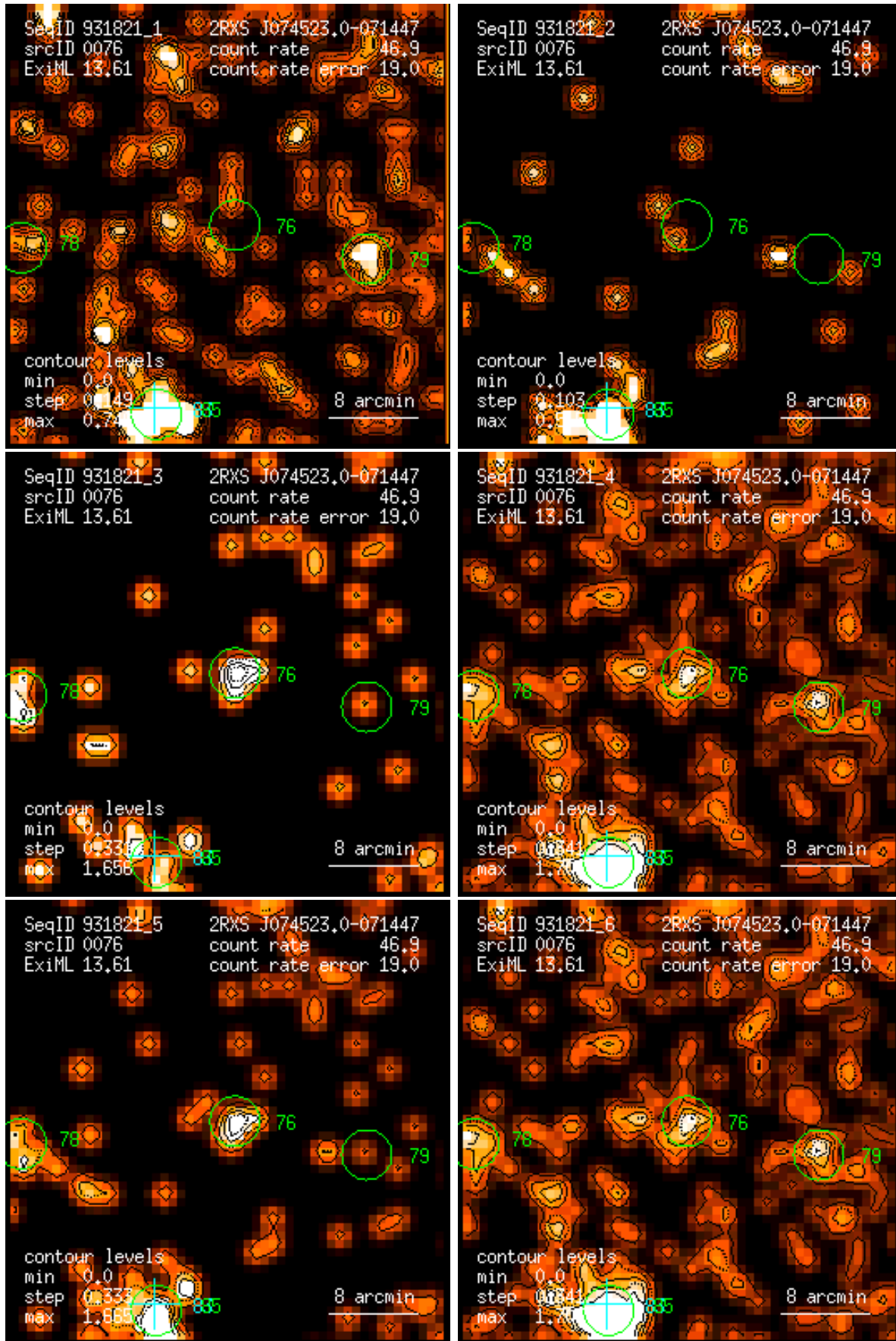
Figure 76: RASS 931821: detection 0076: band rate images, Gaussian filter: (1) PSPC channels 11 – 41, (2) 52 – 90, (3) 91 – 201, (4) 11 – 235, (5) 52 – 201, (6) 11 – 201. Broad band rates in counts/ks. Band rate contour levels in counts/ks/arcmin 2 .
