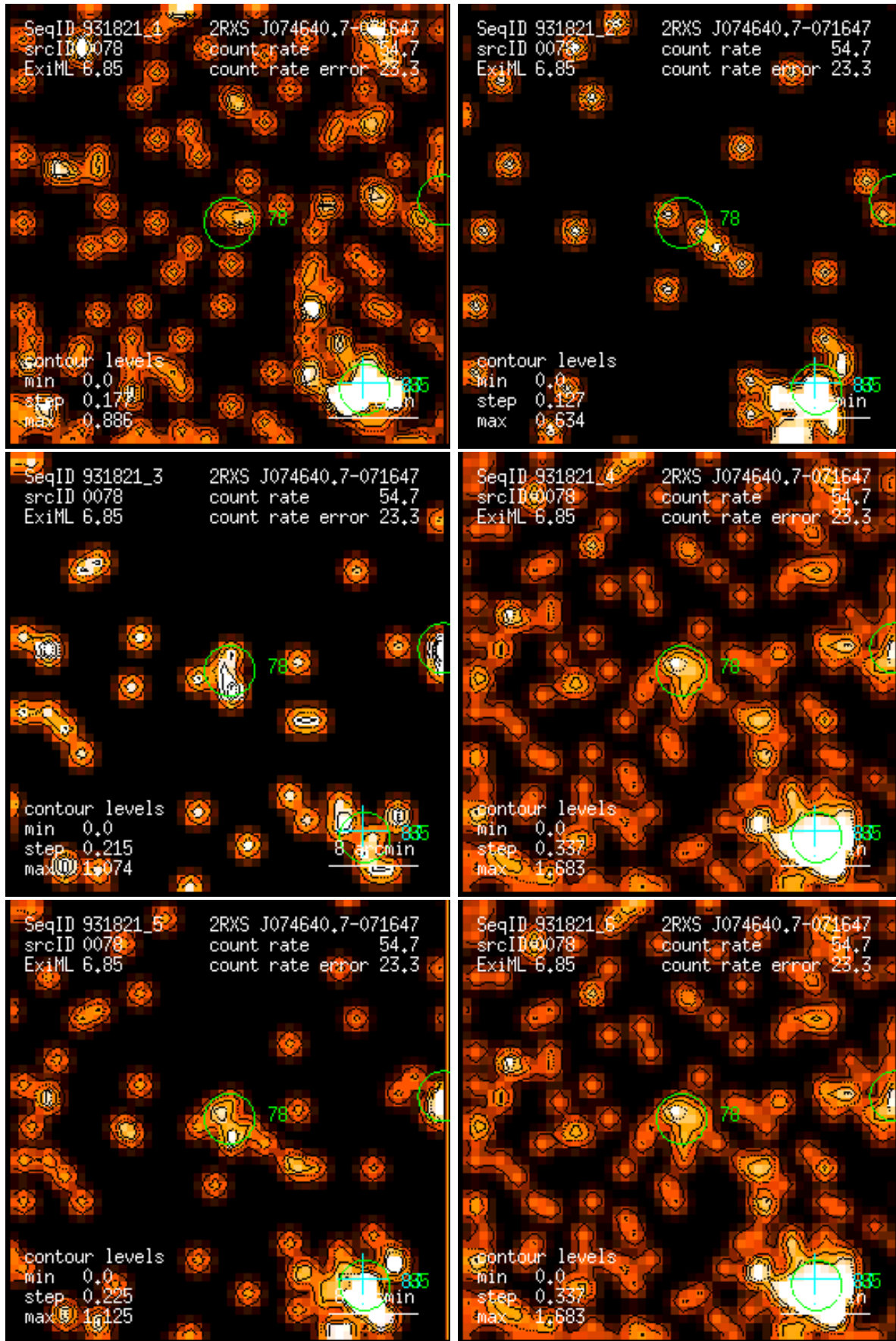
Figure 78: RASS 931821: detection 0078: band rate images, Gaussian filter: (1) PSPC channels 11 – 41, (2) 52 – 90, (3) 91 – 201, (4) 11 – 235, (5) 52 – 201, (6) 11 – 201. Broad band rates in counts/ks. Band rate contour levels in counts/ks/arcmin 2 .
