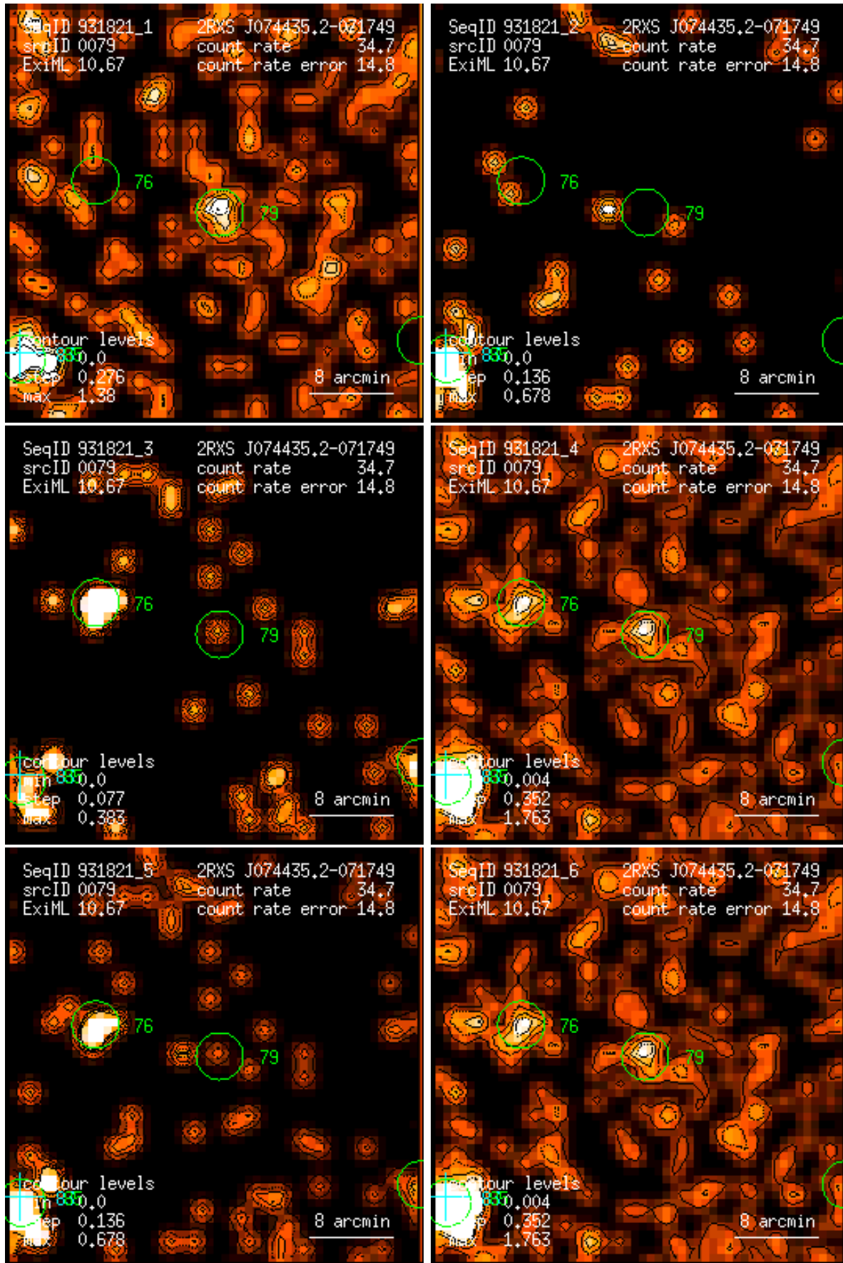
Figure 79: RASS 931821: detection 0079: band rate images, Gaussian filter: (1) PSPC channels 11 – 41, (2) 52 – 90, (3) 91 – 201, (4) 11 – 235, (5) 52 – 201, (6) 11 – 201. Broad band rates in counts/ks. Band rate contour levels in counts/ks/arcmin 2 .
