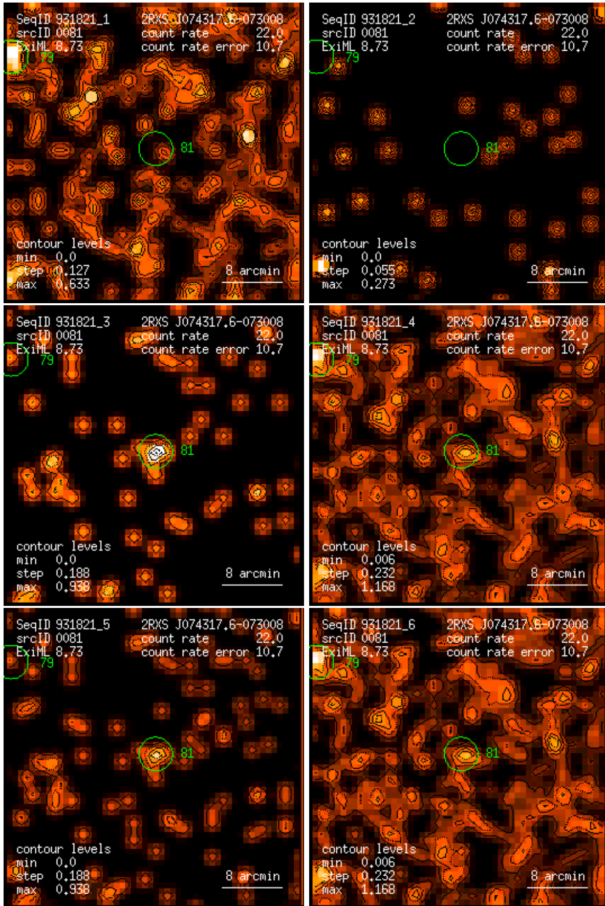
Figure 81: RASS 931821: detection 0081: band rate images, Gaussian filter: (1) PSPC channels 11 – 41, (2) 52 – 90, (3) 91 – 201, (4) 11 – 235, (5) 52 – 201, (6) 11 – 201. Broad band rates in counts/ks. Band rate contour levels in counts/ks/arcmin 2 .
