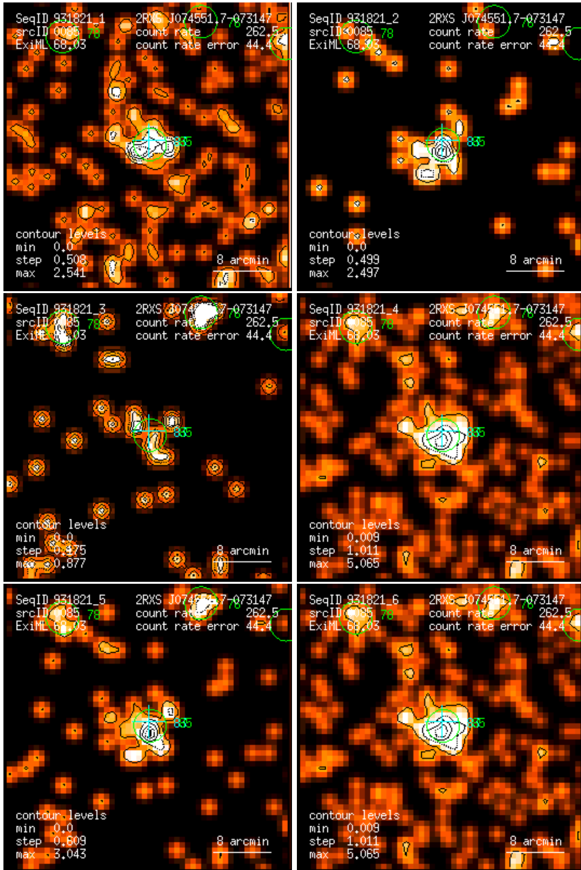
Figure 85: RASS 931821: detection 0085: band rate images, Gaussian filter: (1) PSPC channels 11 – 41, (2) 52 – 90, (3) 91 – 201, (4) 11 – 235, (5) 52 – 201, (6) 11 – 201. Broad band rates in counts/ks. Band rate contour levels in counts/ks/arcmin 2 .
