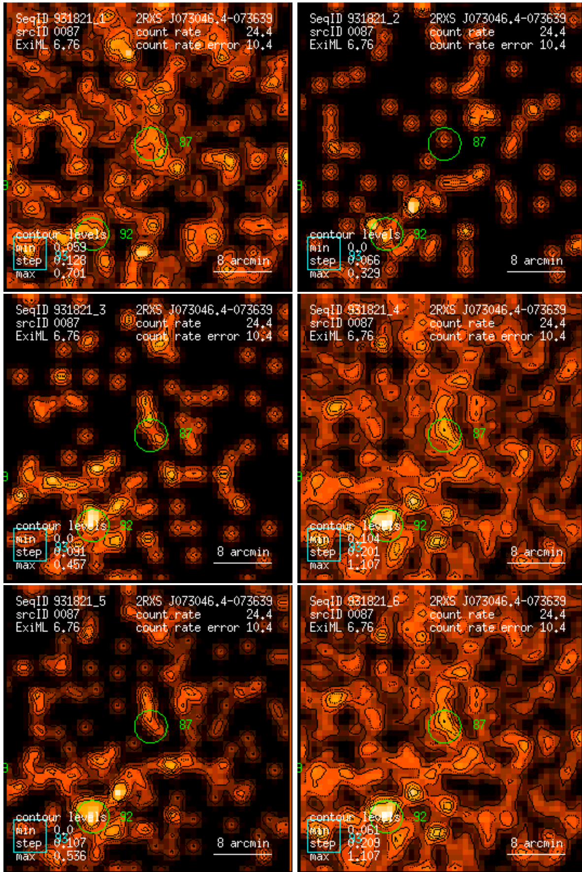
Figure 87: RASS 931821: detection 0087: band rate images, Gaussian filter: (1) PSPC channels 11 – 41, (2) 52 – 90, (3) 91 – 201, (4) 11 – 235, (5) 52 – 201, (6) 11 – 201. Broad band rates in counts/ks. Band rate contour levels in counts/ks/arcmin 2 .
