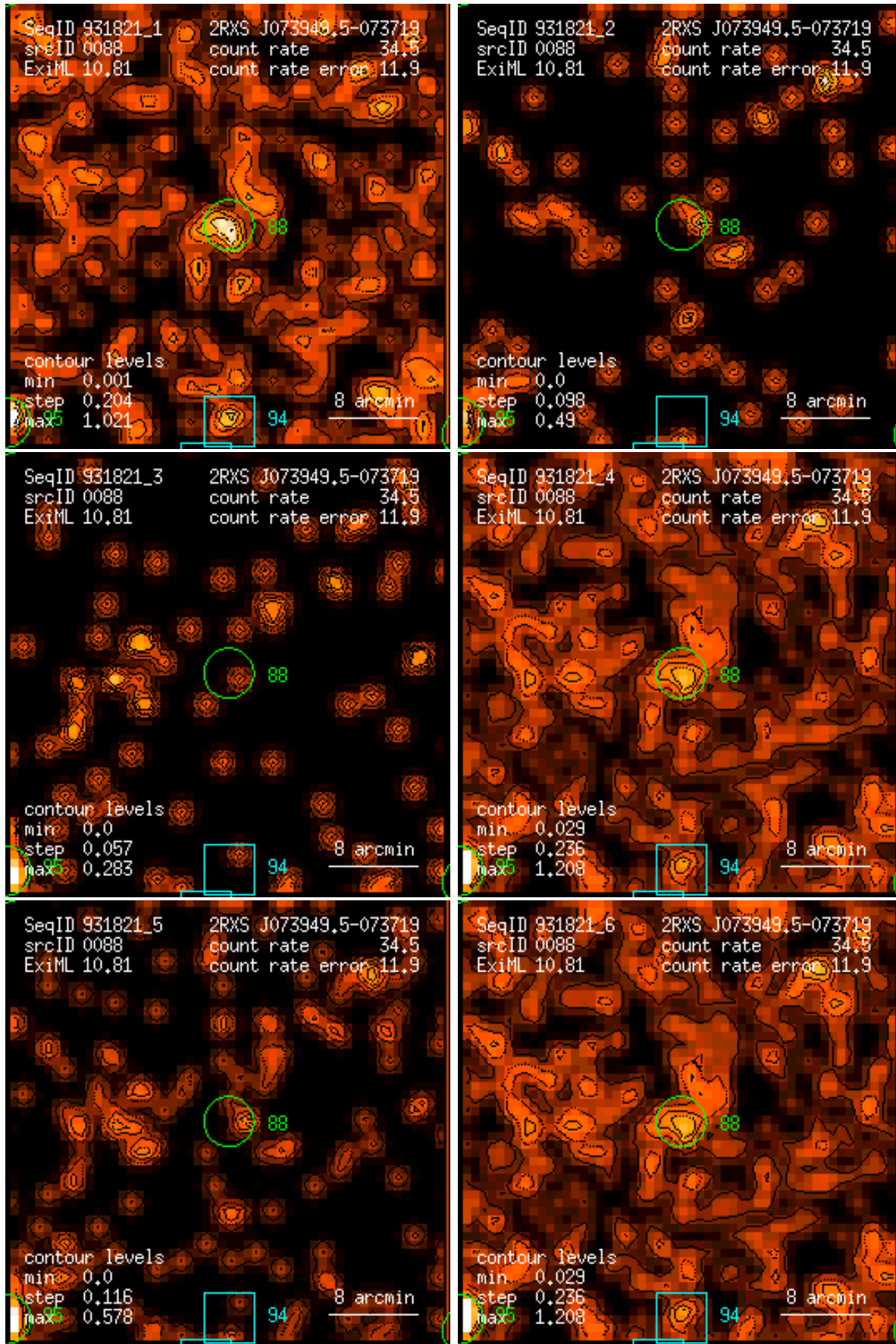
Figure 88: RASS 931821: detection 0088: band rate images, Gaussian filter: (1) PSPC channels 11 – 41, (2) 52 – 90, (3) 91 – 201, (4) 11 – 235, (5) 52 – 201, (6) 11 – 201. Broad band rates in counts/ks. Band rate contour levels in counts/ks/arcmin 2 .
