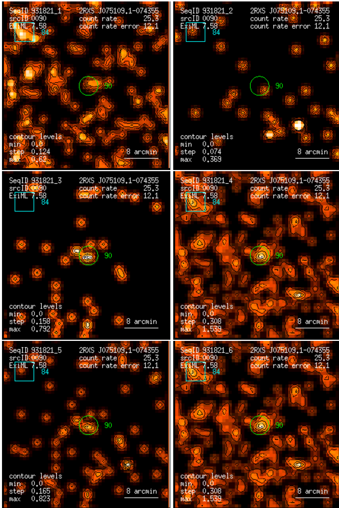
Figure 90: RASS 931821: detection 0090: band rate images, Gaussian filter: (1) PSPC channels 11 – 41, (2) 52 – 90, (3) 91 – 201, (4) 11 – 235, (5) 52 – 201, (6) 11 – 201. Broad band rates in counts/ks. Band rate contour levels in counts/ks/arcmin 2 .
