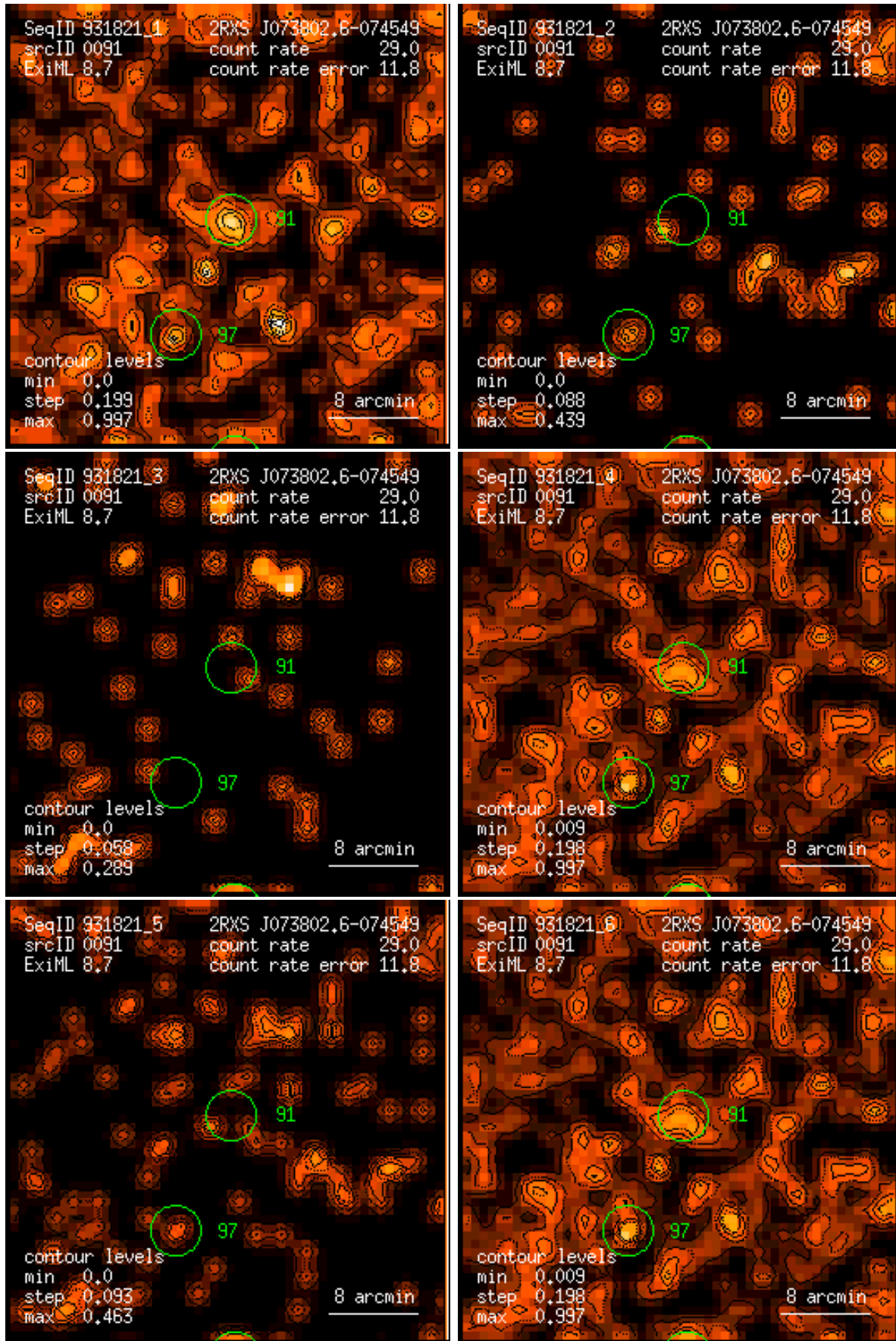
Figure 91: RASS 931821: detection 0091: band rate images, Gaussian filter: (1) PSPC channels 11 – 41, (2) 52 – 90, (3) 91 – 201, (4) 11 – 235, (5) 52 – 201, (6) 11 – 201. Broad band rates in counts/ks. Band rate contour levels in counts/ks/arcmin 2 .
