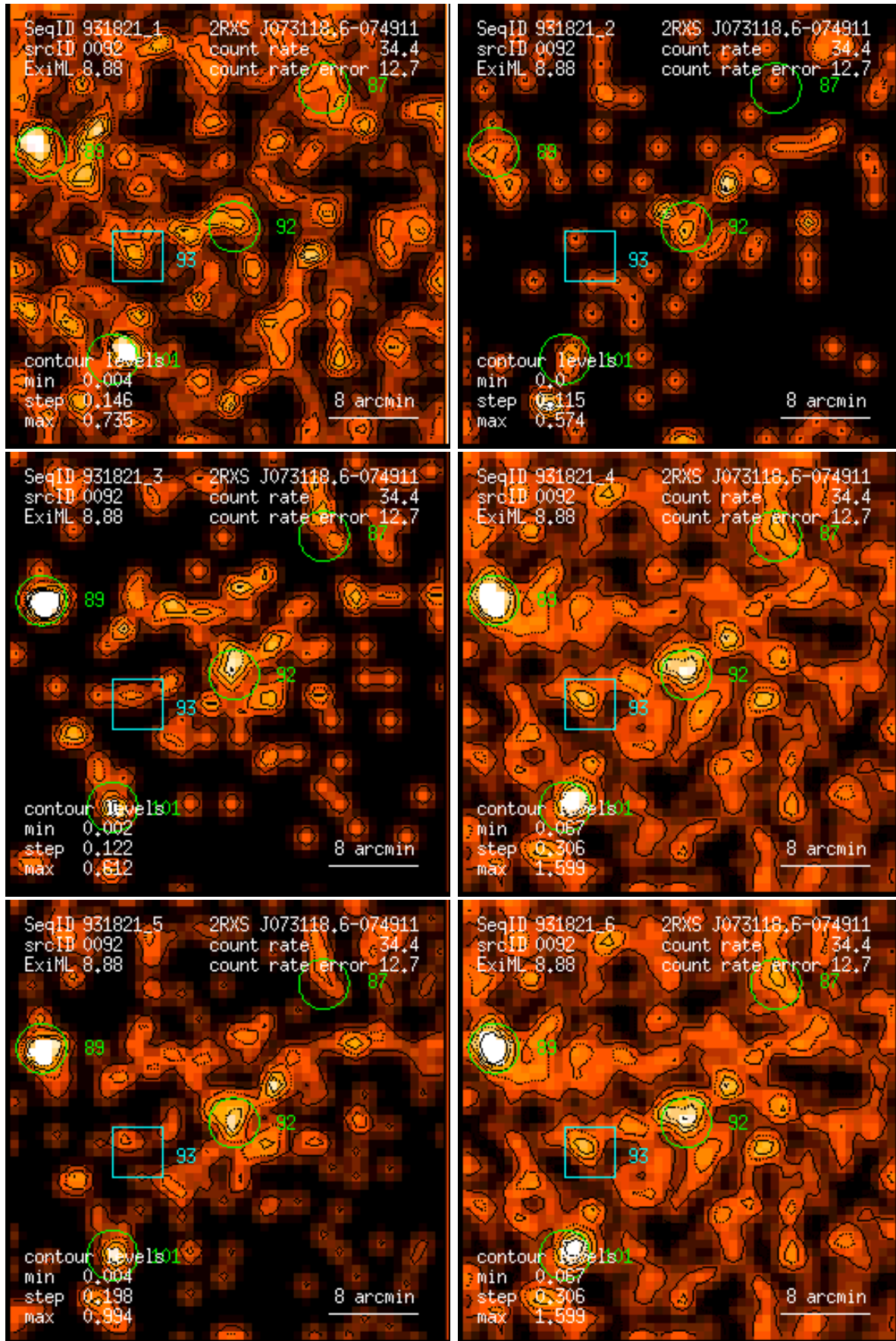
Figure 92: RASS 931821: detection 0092: band rate images, Gaussian filter: (1) PSPC channels 11 – 41, (2) 52 – 90, (3) 91 – 201, (4) 11 – 235, (5) 52 – 201, (6) 11 – 201. Broad band rates in counts/ks. Band rate contour levels in counts/ks/arcmin 2 .
