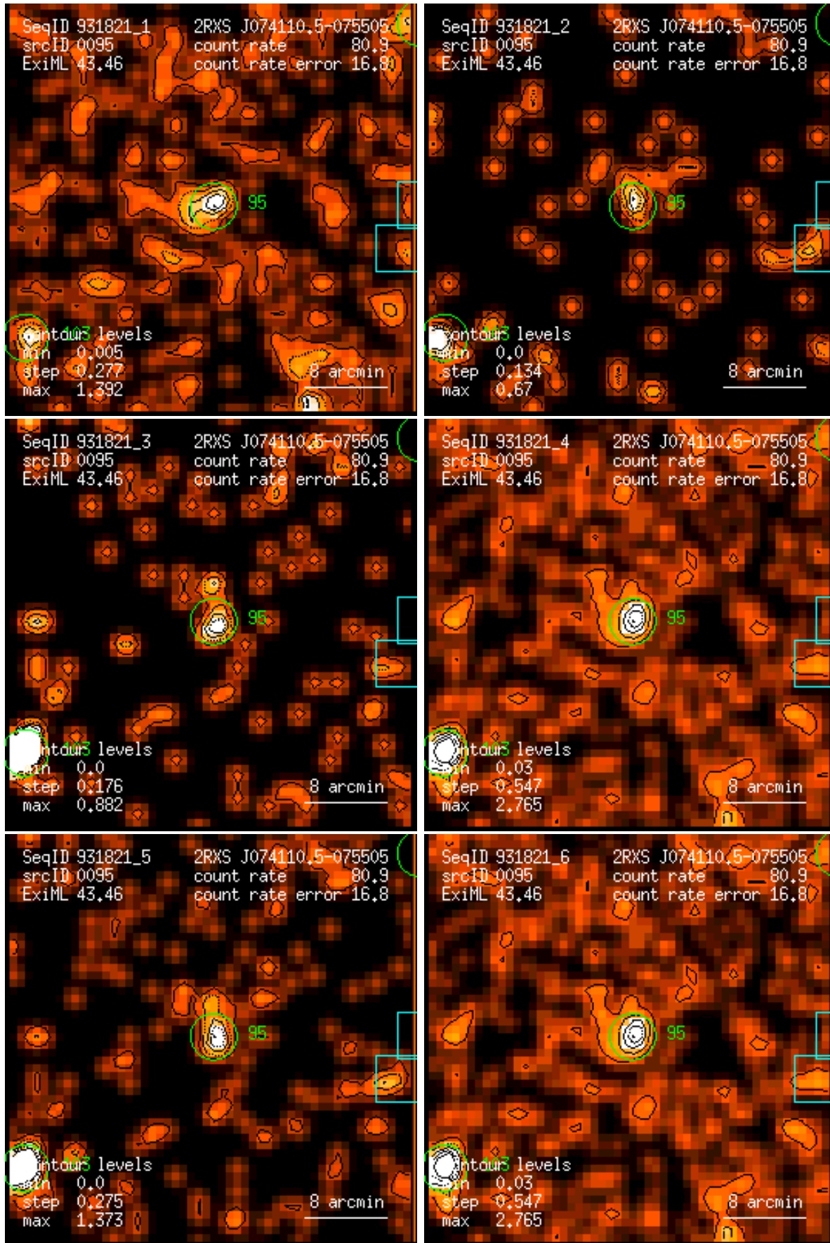
Figure 95: RASS 931821: detection 0095: band rate images, Gaussian filter: (1) PSPC channels 11 – 41, (2) 52 – 90, (3) 91 – 201, (4) 11 – 235, (5) 52 – 201, (6) 11 – 201. Broad band rates in counts/ks. Band rate contour levels in counts/ks/arcmin 2 .
