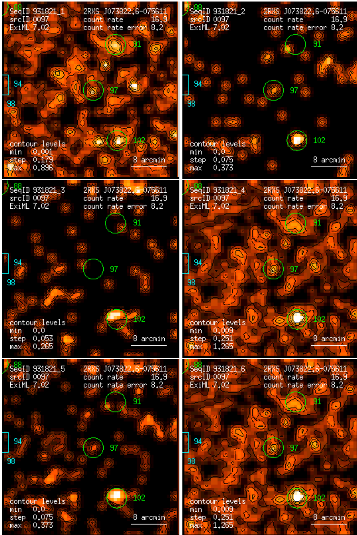
Figure 97: RASS 931821: detection 0097: band rate images, Gaussian filter: (1) PSPC channels 11 – 41, (2) 52 – 90, (3) 91 – 201, (4) 11 – 235, (5) 52 – 201, (6) 11 – 201. Broad band rates in counts/ks. Band rate contour levels in counts/ks/arcmin 2 .
