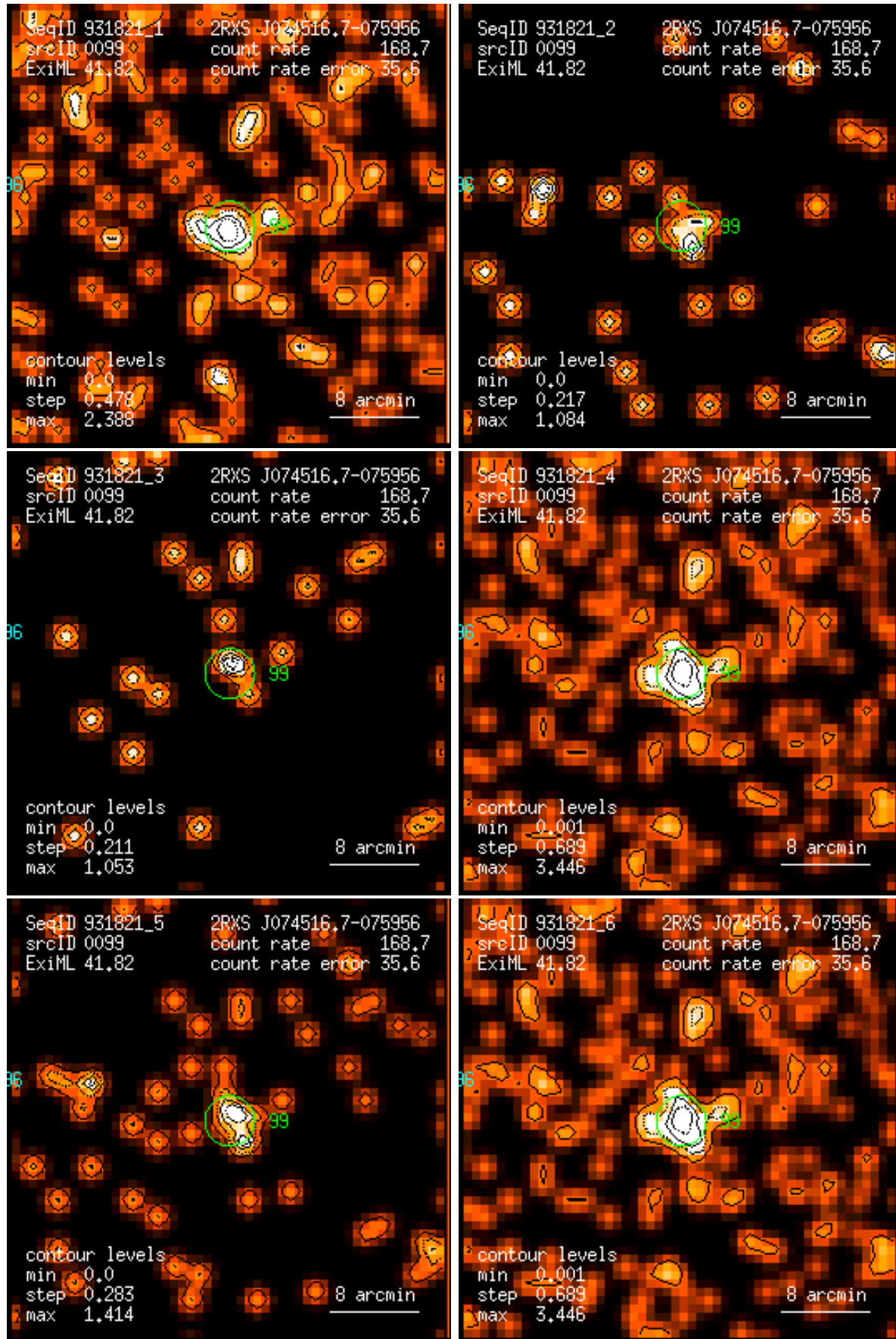
Figure 99: RASS 931821: detection 0099: band rate images, Gaussian filter: (1) PSPC channels 11 – 41, (2) 52 – 90, (3) 91 – 201, (4) 11 – 235, (5) 52 – 201, (6) 11 – 201. Broad band rates in counts/ks. Band rate contour levels in counts/ks/arcmin 2 .
