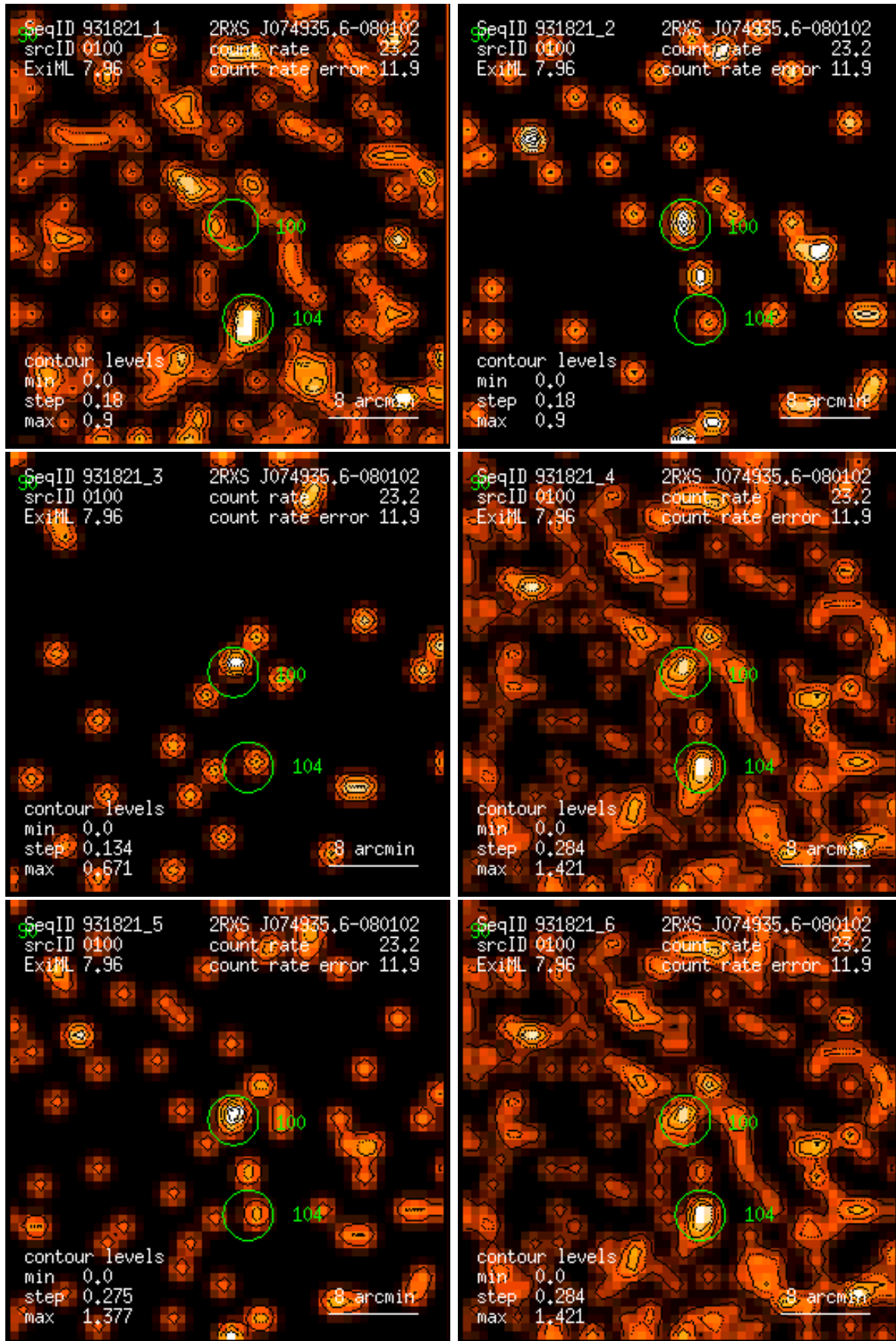
Figure 100: RASS 931821: detection 0100: band rate images, Gaussian filter: (1) PSPC channels 11 – 41, (2) 52 – 90, (3) 91 – 201, (4) 11 – 235, (5) 52 – 201, (6) 11 – 201. Broad band rates in counts/ks. Band rate contour levels in counts/ks/arcmin 2 .
