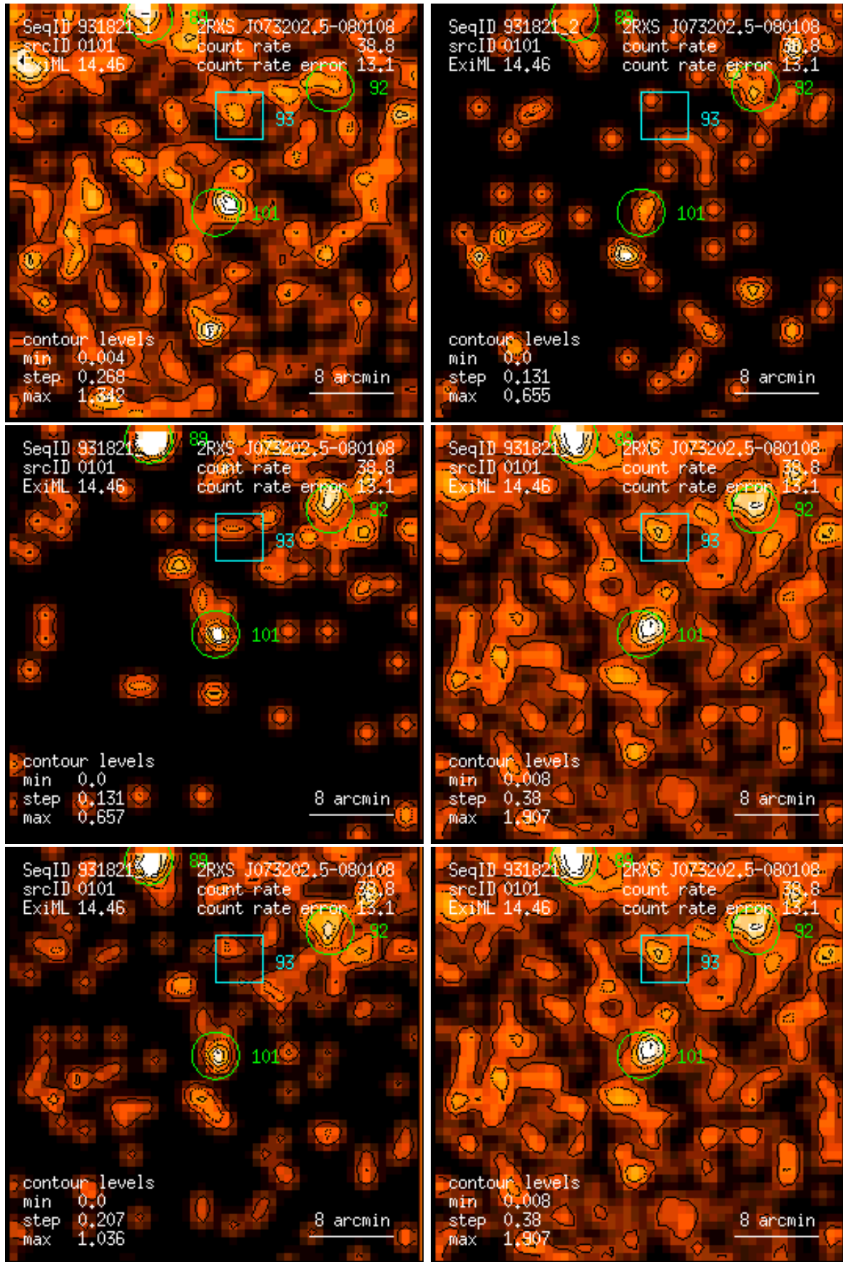
Figure 101: RASS 931821: detection 0101: band rate images, Gaussian filter: (1) PSPC channels 11 – 41, (2) 52 – 90, (3) 91 – 201, (4) 11 – 235, (5) 52 – 201, (6) 11 – 201. Broad band rates in counts/ks. Band rate contour levels in counts/ks/arcmin 2 .
