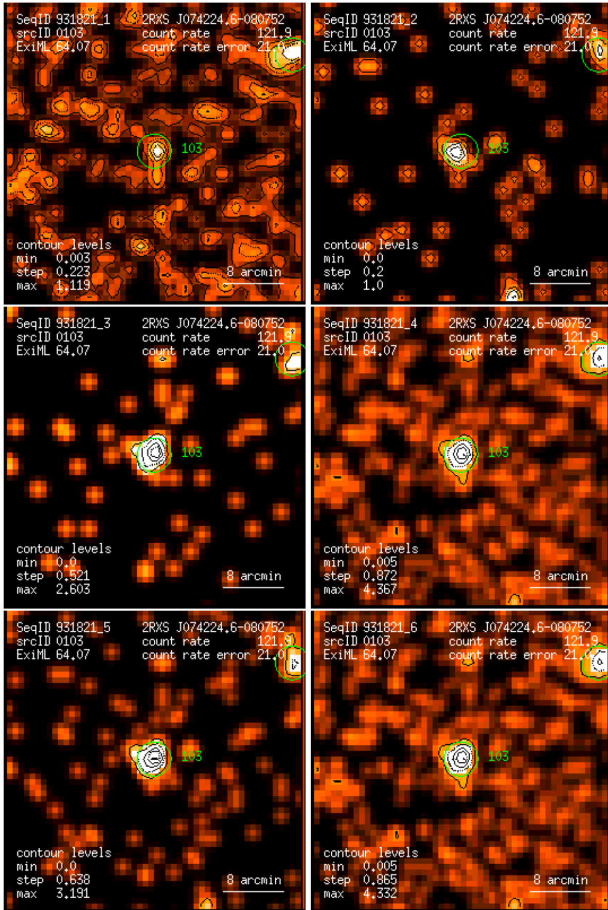
Figure 103: RASS 931821: detection 0103: band rate images, Gaussian filter: (1) PSPC channels 11 – 41, (2) 52 – 90, (3) 91 – 201, (4) 11 – 235, (5) 52 – 201, (6) 11 – 201. Broad band rates in counts/ks. Band rate contour levels in counts/ks/arcmin 2 .
