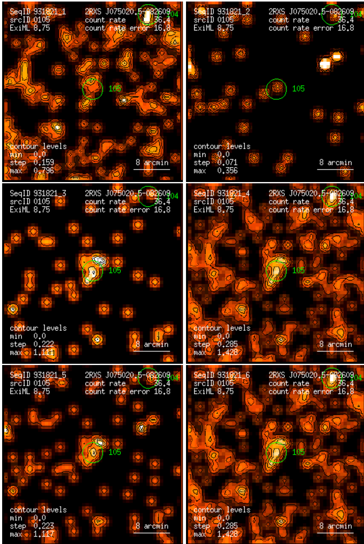
Figure 105: RASS 931821: detection 0105: band rate images, Gaussian filter: (1) PSPC channels 11 – 41, (2) 52 – 90, (3) 91 – 201, (4) 11 – 235, (5) 52 – 201, (6) 11 – 201. Broad band rates in counts/ks. Band rate contour levels in counts/ks/arcmin 2 .
