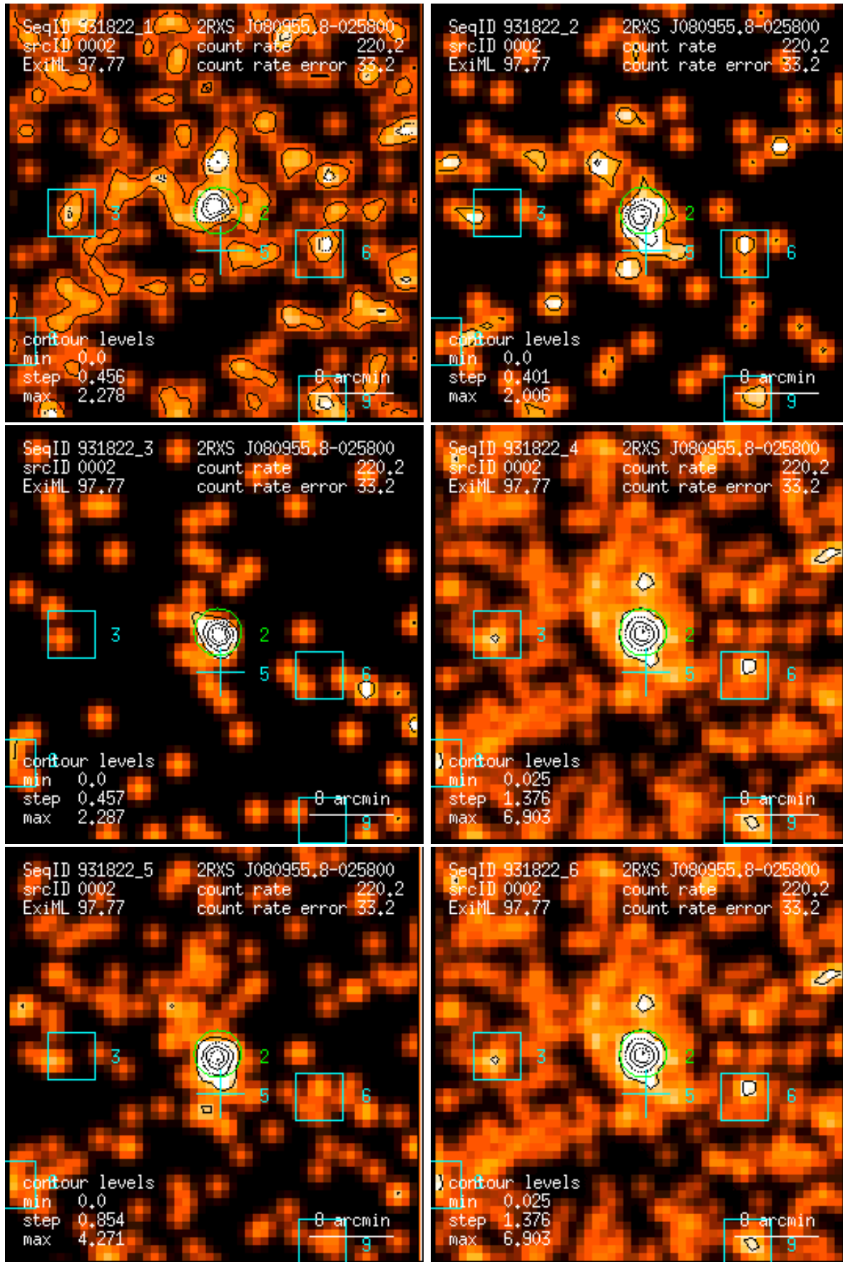
Figure 2: RASS 931822: detection 0002: band rate images, Gaussian filter: (1) PSPC channels 11 – 41, (2) 52 – 90, (3) 91 – 201, (4) 11 – 235, (5) 52 – 201, (6) 11 – 201. Broad band rates in counts/ks. Band rate contour levels in counts/ks/arcmin 2 .
