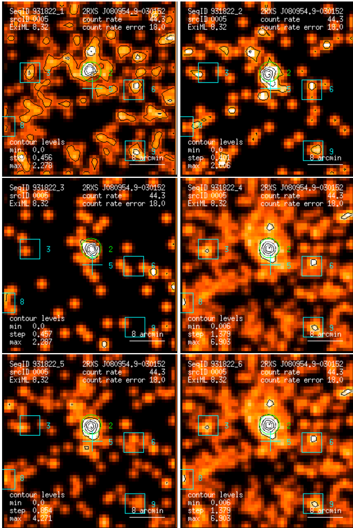
Figure 5: RASS 931822: detection 0005: band rate images, Gaussian filter: (1) PSPC channels 11 – 41, (2) 52 – 90, (3) 91 – 201, (4) 11 – 235, (5) 52 – 201, (6) 11 – 201. Broad band rates in counts/ks. Band rate contour levels in counts/ks/arcmin 2 .
