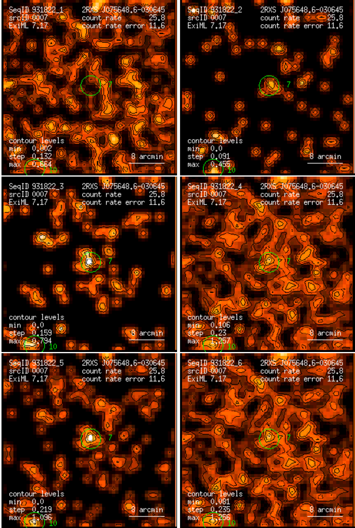
Figure 7: RASS 931822: detection 0007: band rate images, Gaussian filter: (1) PSPC channels 11 – 41, (2) 52 – 90, (3) 91 – 201, (4) 11 – 235, (5) 52 – 201, (6) 11 – 201. Broad band rates in counts/ks. Band rate contour levels in counts/ks/arcmin 2 .
