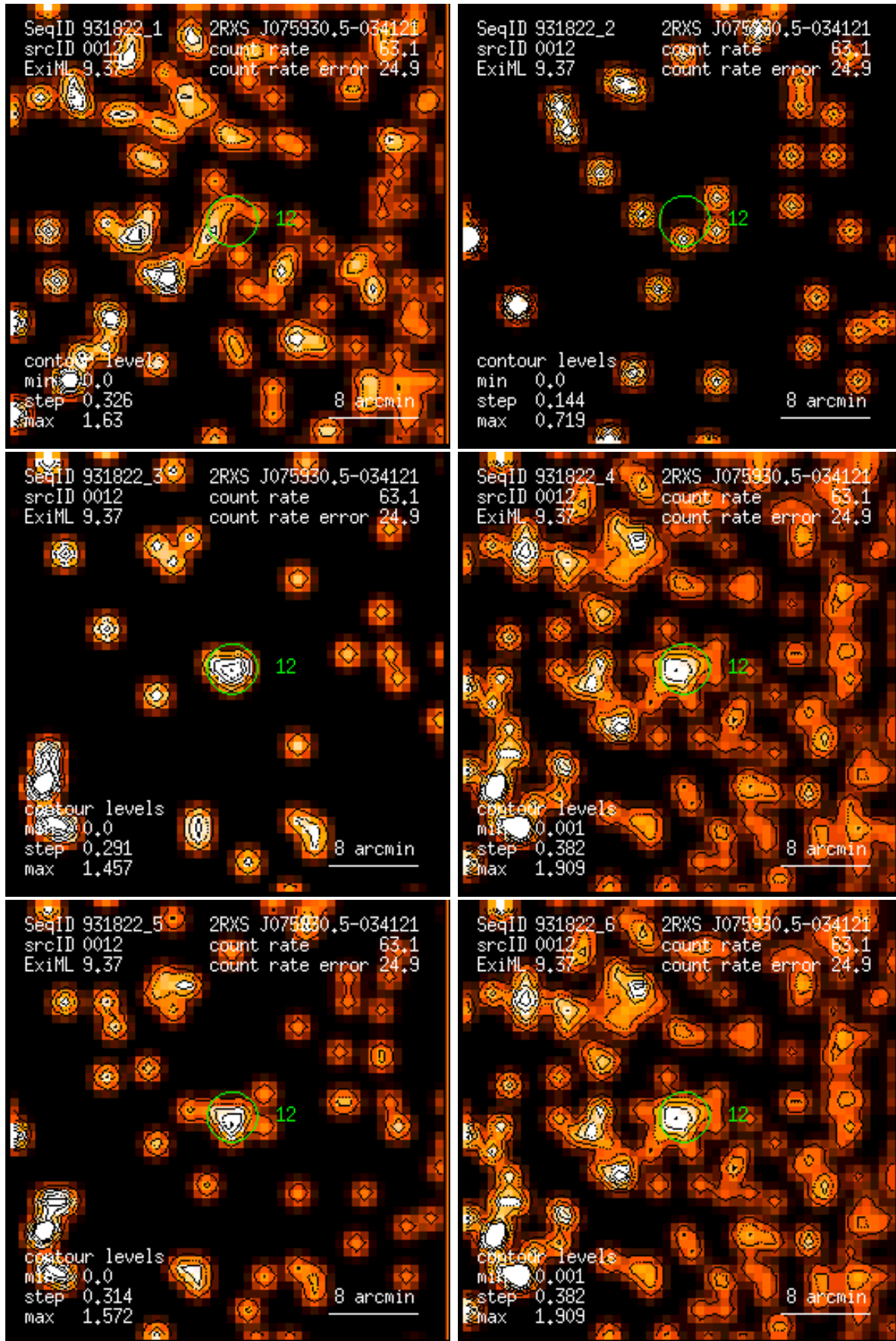
Figure 12: RASS 931822: detection 0012: band rate images, Gaussian filter: (1) PSPC channels 11 – 41, (2) 52 – 90, (3) 91 – 201, (4) 11 – 235, (5) 52 – 201, (6) 11 – 201. Broad band rates in counts/ks. Band rate contour levels in counts/ks/arcmin 2 .
