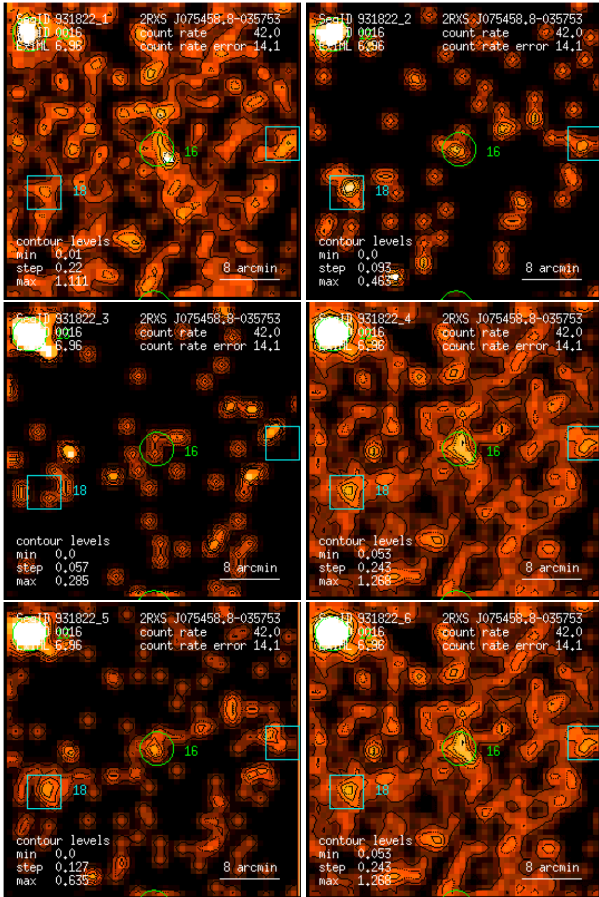
Figure 16: RASS 931822: detection 0016: band rate images, Gaussian filter: (1) PSPC channels 11 – 41, (2) 52 – 90, (3) 91 – 201, (4) 11 – 235, (5) 52 – 201, (6) 11 – 201. Broad band rates in counts/ks. Band rate contour levels in counts/ks/arcmin 2 .
