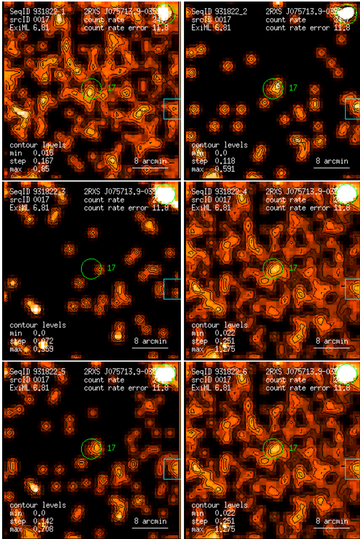
Figure 17: RASS 931822: detection 0017: band rate images, Gaussian filter: (1) PSPC channels 11 – 41, (2) 52 – 90, (3) 91 – 201, (4) 11 – 235, (5) 52 – 201, (6) 11 – 201. Broad band rates in counts/ks. Band rate contour levels in counts/ks/arcmin 2 .
