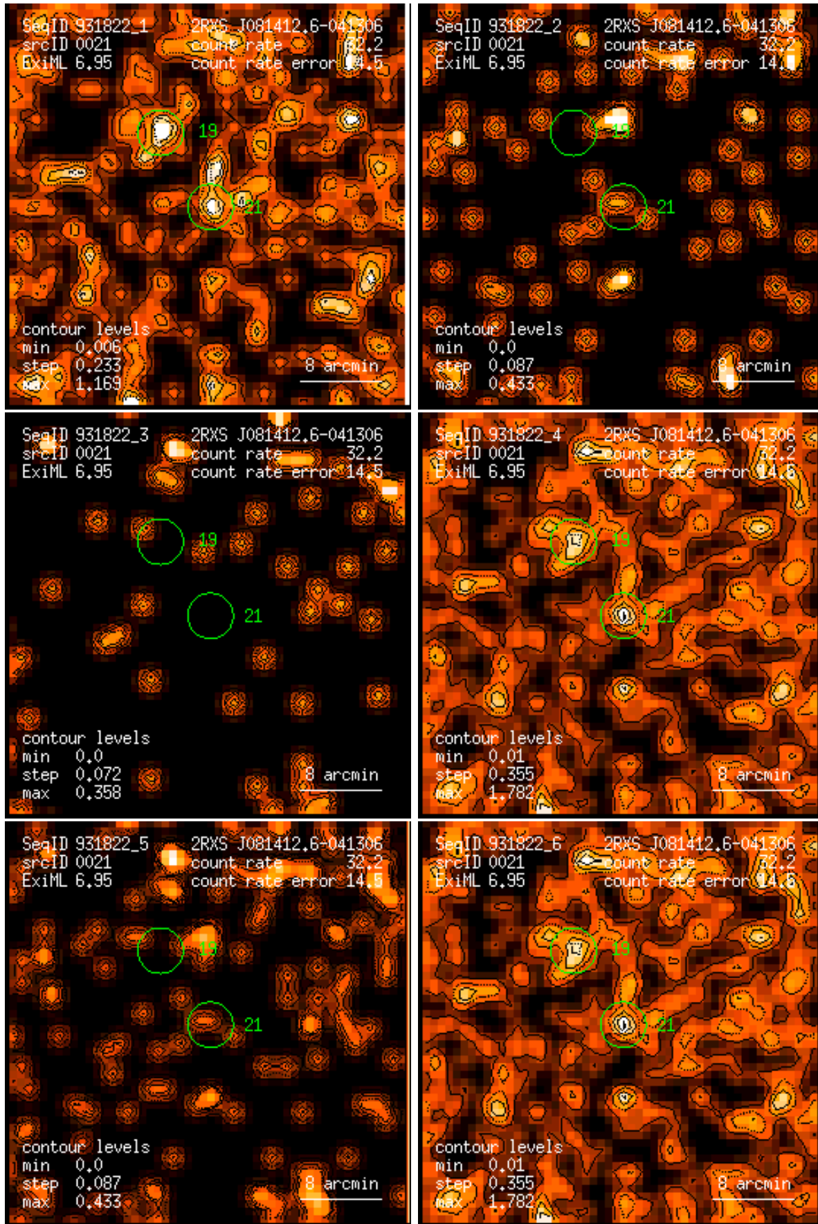
Figure 21: RASS 931822: detection 0021: band rate images, Gaussian filter: (1) PSPC channels 11 – 41, (2) 52 – 90, (3) 91 – 201, (4) 11 – 235, (5) 52 – 201, (6) 11 – 201. Broad band rates in counts/ks. Band rate contour levels in counts/ks/arcmin 2 .
