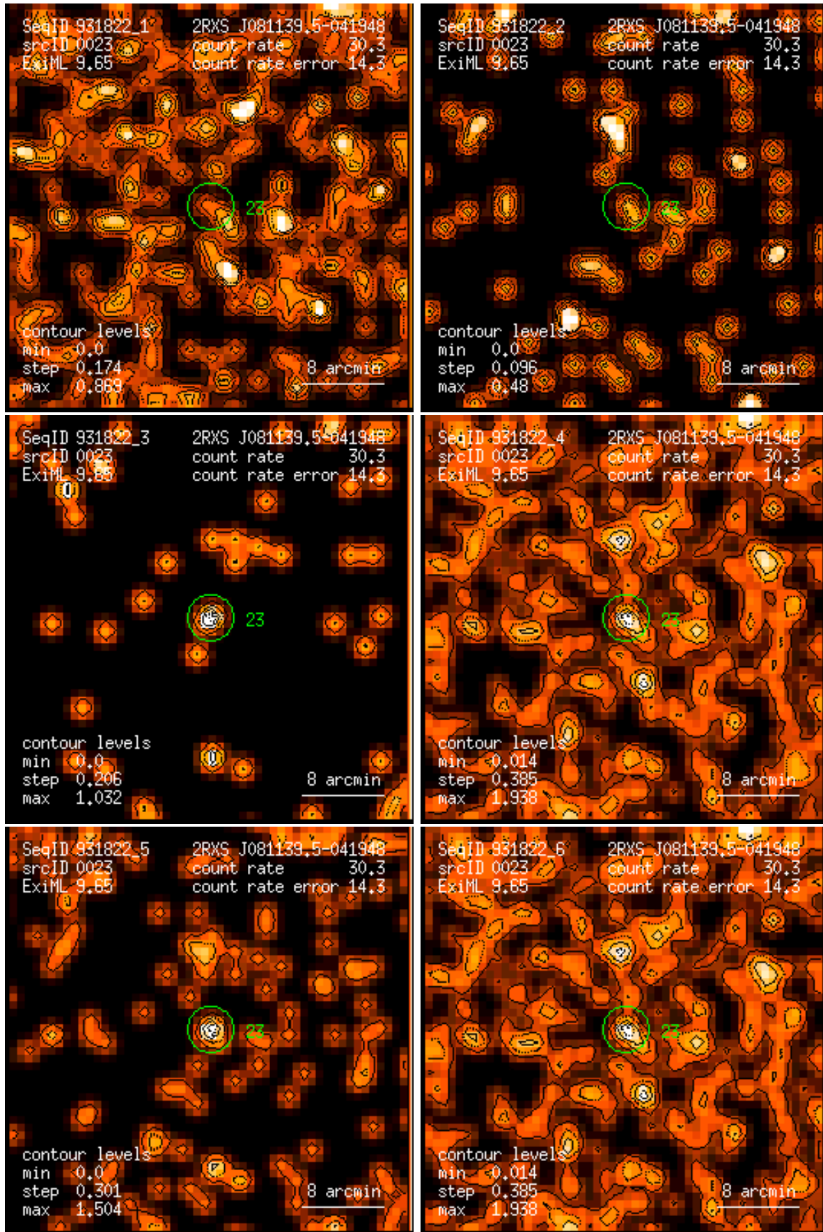
Figure 23: RASS 931822: detection 0023: band rate images, Gaussian filter: (1) PSPC channels 11 – 41, (2) 52 – 90, (3) 91 – 201, (4) 11 – 235, (5) 52 – 201, (6) 11 – 201. Broad band rates in counts/ks. Band rate contour levels in counts/ks/arcmin 2 .
