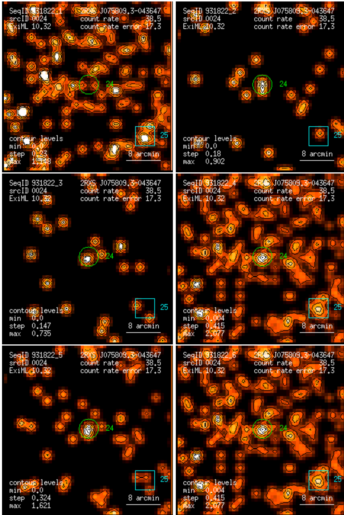
Figure 24: RASS 931822: detection 0024: band rate images, Gaussian filter: (1) PSPC channels 11 – 41, (2) 52 – 90, (3) 91 – 201, (4) 11 – 235, (5) 52 – 201, (6) 11 – 201. Broad band rates in counts/ks. Band rate contour levels in counts/ks/arcmin 2 .
