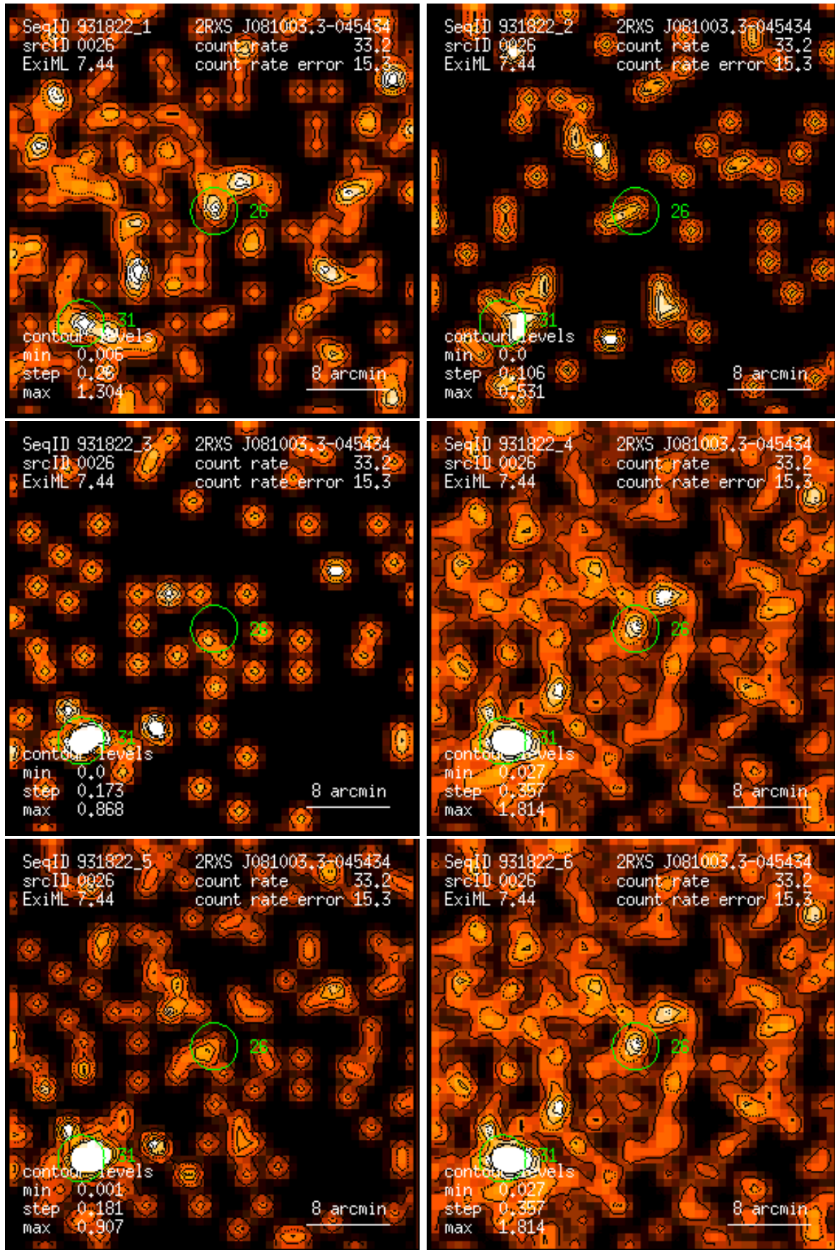
Figure 26: RASS 931822: detection 0026: band rate images, Gaussian filter: (1) PSPC channels 11 – 41, (2) 52 – 90, (3) 91 – 201, (4) 11 – 235, (5) 52 – 201, (6) 11 – 201. Broad band rates in counts/ks. Band rate contour levels in counts/ks/arcmin 2 .
