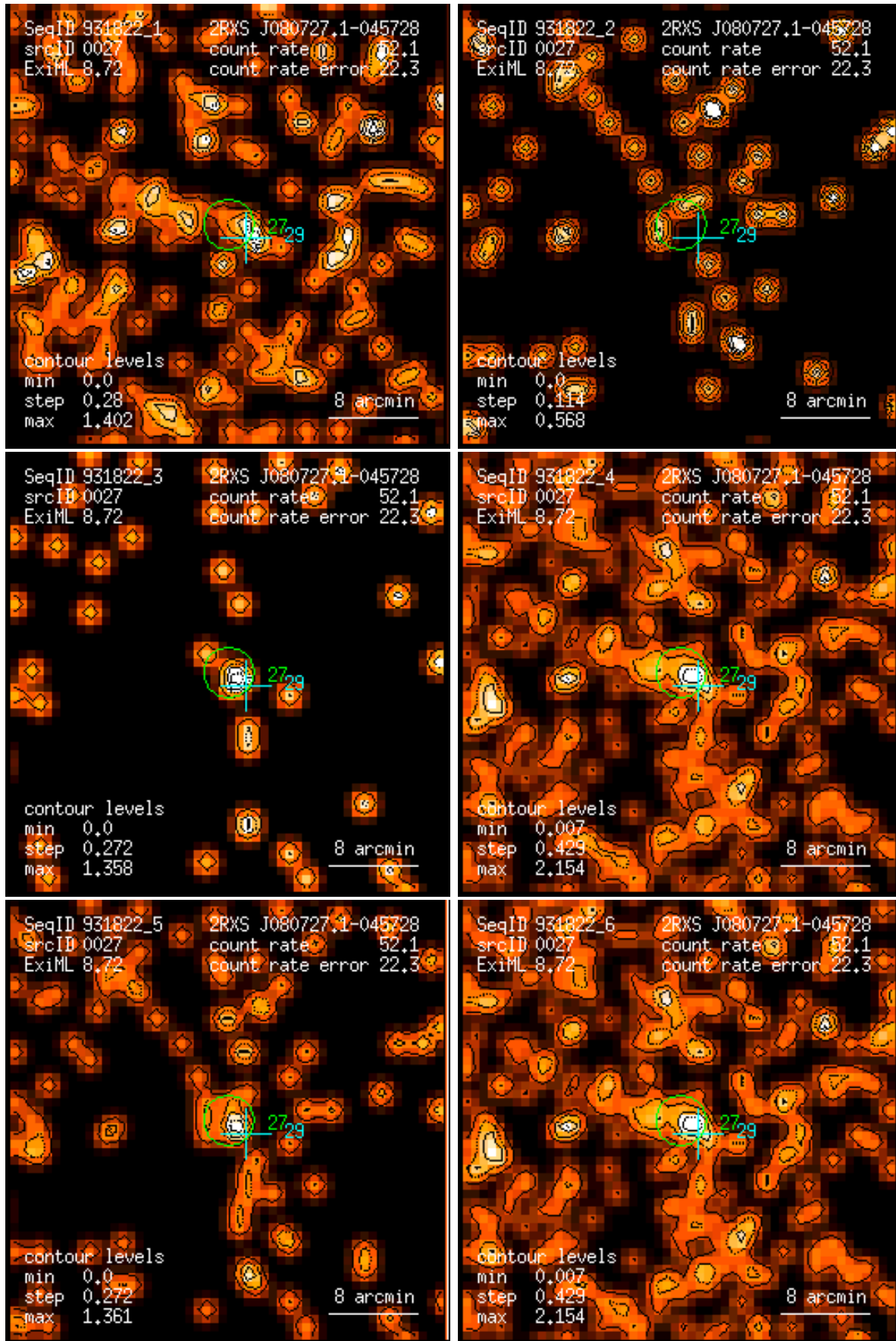
Figure 27: RASS 931822: detection 0027: band rate images, Gaussian filter: (1) PSPC channels 11 – 41, (2) 52 – 90, (3) 91 – 201, (4) 11 – 235, (5) 52 – 201, (6) 11 – 201. Broad band rates in counts/ks. Band rate contour levels in counts/ks/arcmin 2 .
