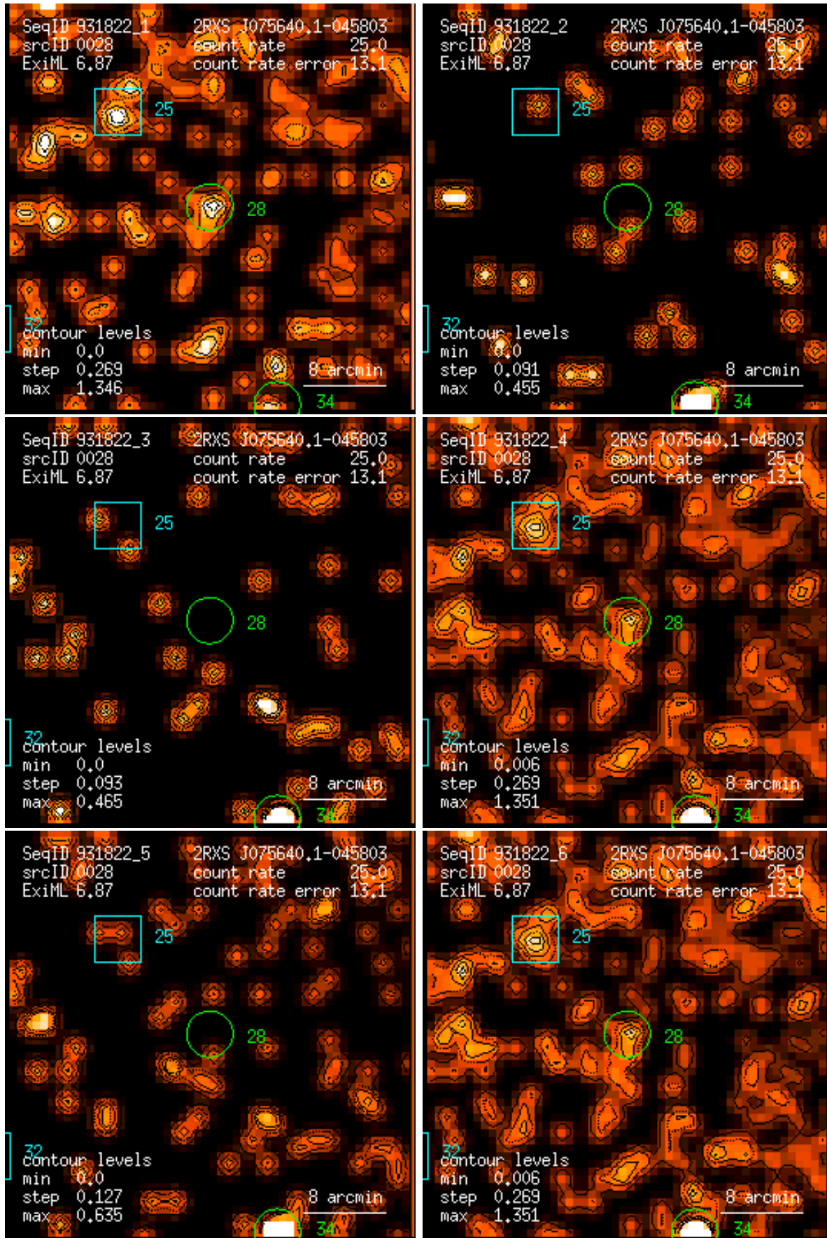
Figure 28: RASS 931822: detection 0028: band rate images, Gaussian filter: (1) PSPC channels 11 – 41, (2) 52 – 90, (3) 91 – 201, (4) 11 – 235, (5) 52 – 201, (6) 11 – 201. Broad band rates in counts/ks. Band rate contour levels in counts/ks/arcmin 2 .
