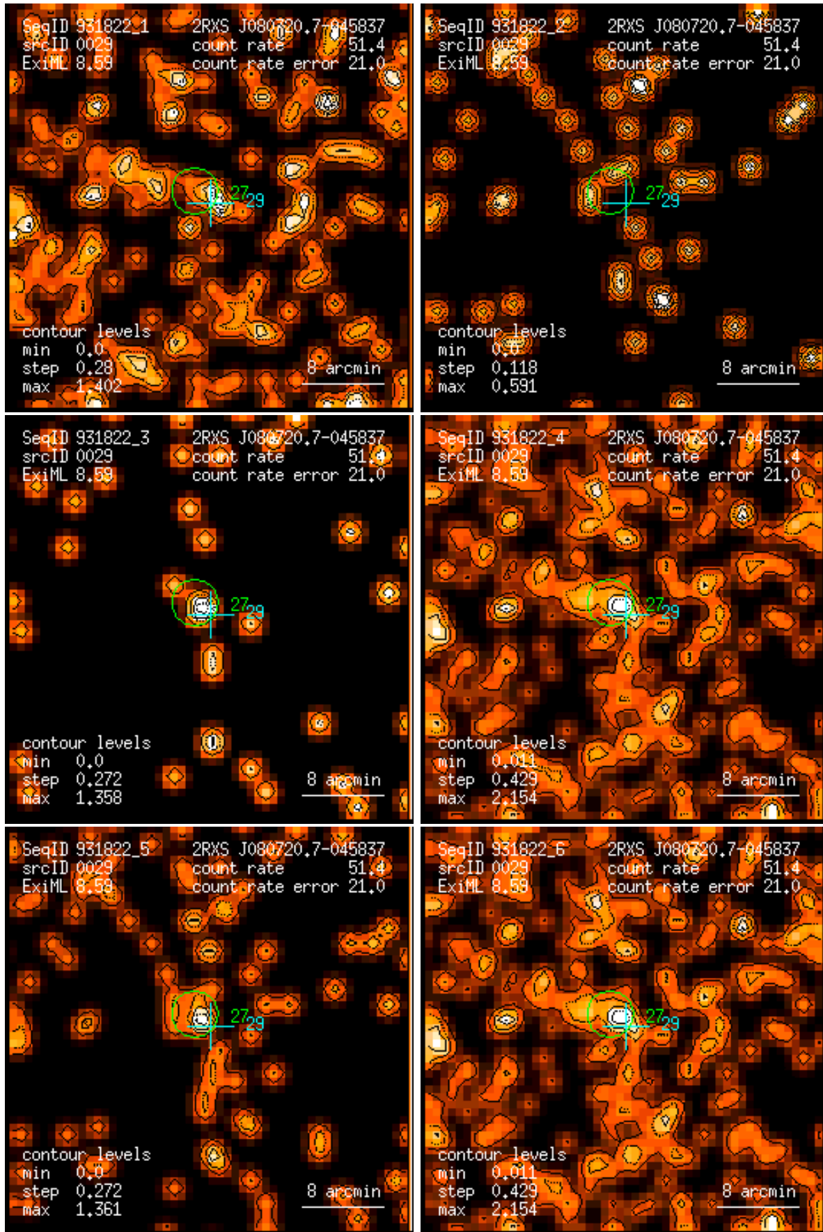
Figure 29: RASS 931822: detection 0029: band rate images, Gaussian filter: (1) PSPC channels 11 – 41, (2) 52 – 90, (3) 91 – 201, (4) 11 – 235, (5) 52 – 201, (6) 11 – 201. Broad band rates in counts/ks. Band rate contour levels in counts/ks/arcmin 2 .
