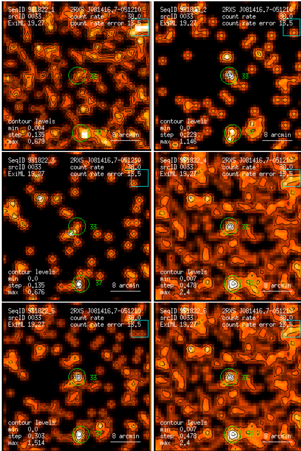
Figure 33: RASS 931822: detection 0033: band rate images, Gaussian filter: (1) PSPC channels 11 – 41, (2) 52 – 90, (3) 91 – 201, (4) 11 – 235, (5) 52 – 201, (6) 11 – 201. Broad band rates in counts/ks. Band rate contour levels in counts/ks/arcmin 2 .
