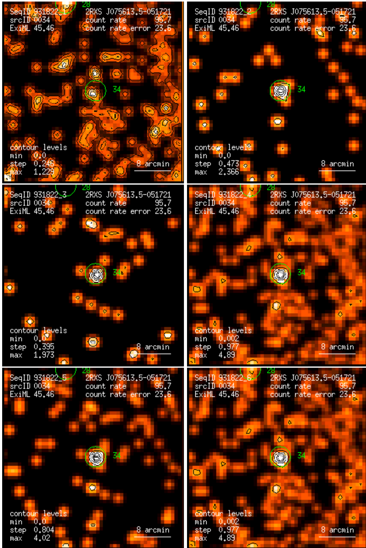
Figure 34: RASS 931822: detection 0034: band rate images, Gaussian filter: (1) PSPC channels 11 – 41, (2) 52 – 90, (3) 91 – 201, (4) 11 – 235, (5) 52 – 201, (6) 11 – 201. Broad band rates in counts/ks. Band rate contour levels in counts/ks/arcmin 2 .
