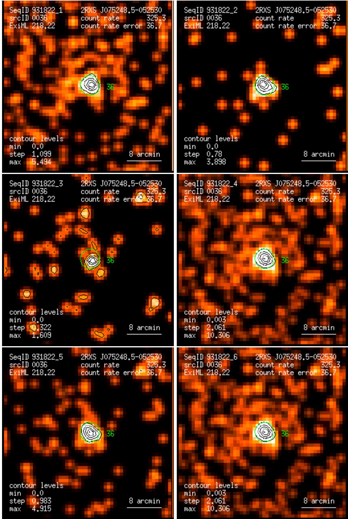
Figure 36: RASS 931822: detection 0036: band rate images, Gaussian filter: (1) PSPC channels 11 – 41, (2) 52 – 90, (3) 91 – 201, (4) 11 – 235, (5) 52 – 201, (6) 11 – 201. Broad band rates in counts/ks. Band rate contour levels in counts/ks/arcmin 2 .
