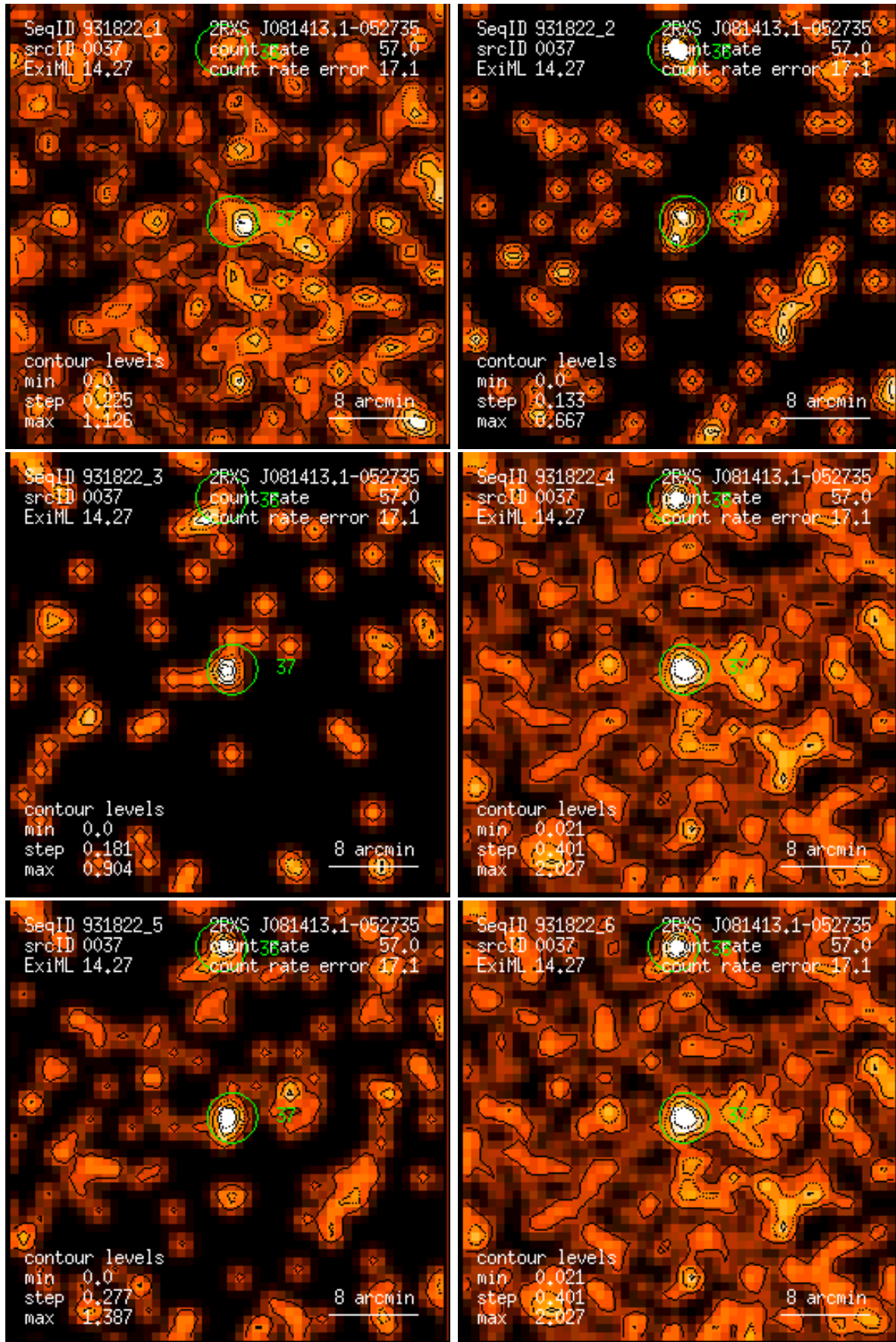
Figure 37: RASS 931822: detection 0037: band rate images, Gaussian filter: (1) PSPC channels 11 – 41, (2) 52 – 90, (3) 91 – 201, (4) 11 – 235, (5) 52 – 201, (6) 11 – 201. Broad band rates in counts/ks. Band rate contour levels in counts/ks/arcmin 2 .
